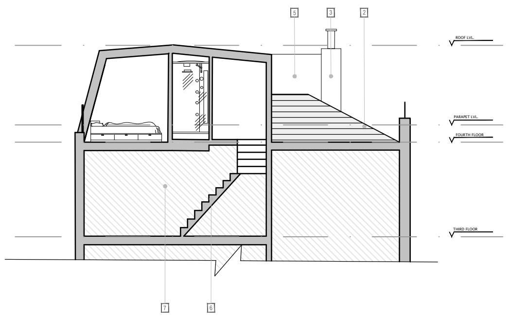
6 SECTION BB EXISTING 1:100
