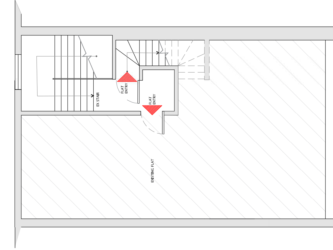
2 THIRD FLOOR PLAN 1:50 EXISTING
