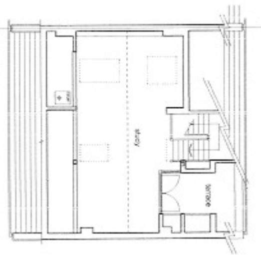
second - as proposed
