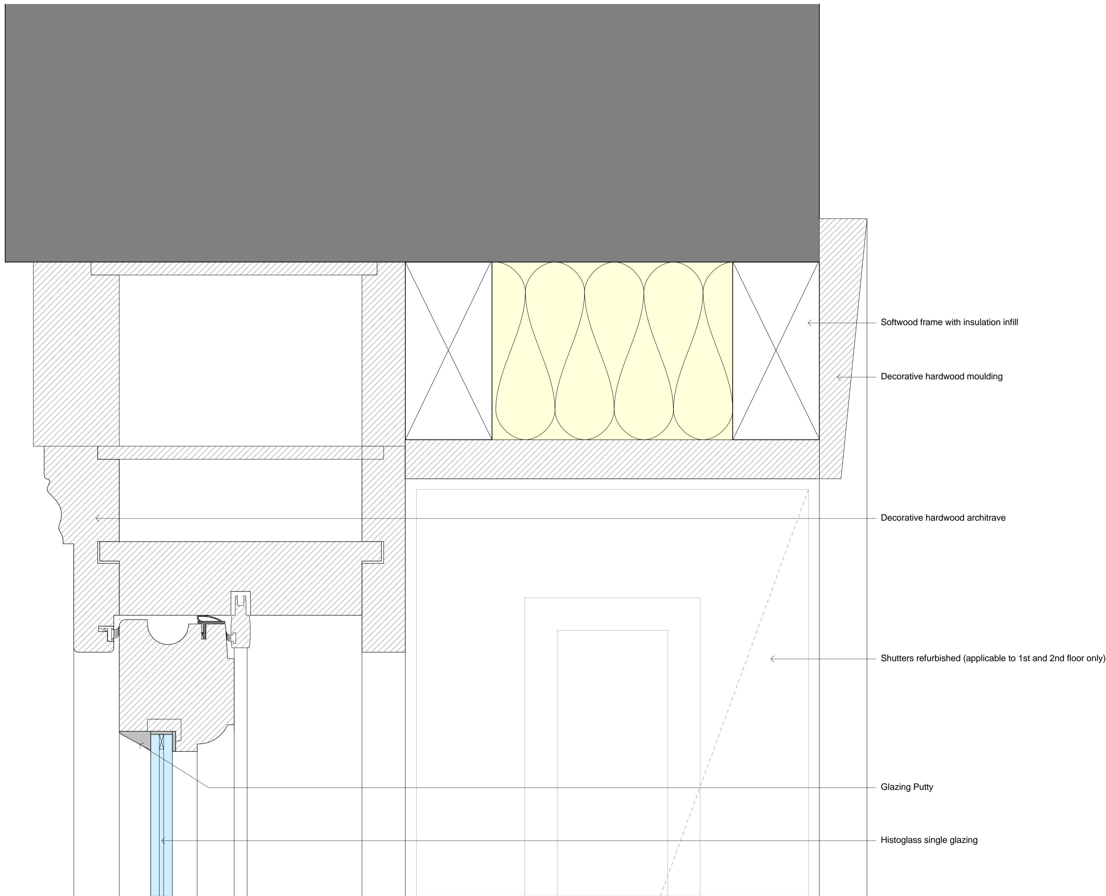
1 26 Denmark Street Typical North Architrave and Moulding Details (Window Type L) Scale: 1 : 1
