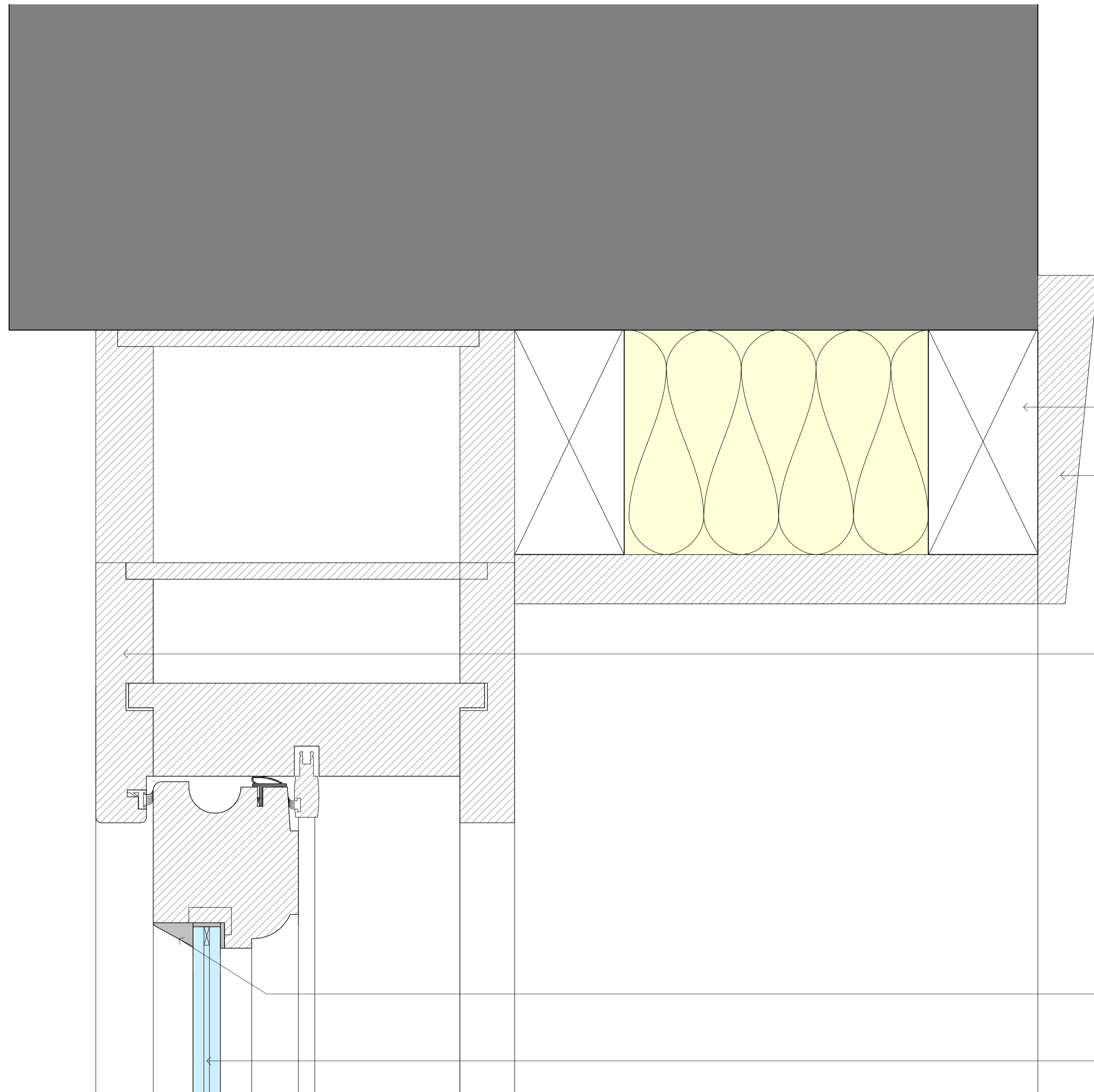
1 26 Denmark Street Typical South Architrave and Moulding Details (Window Types O, P, P1 & N) Scale: 1 : 1
