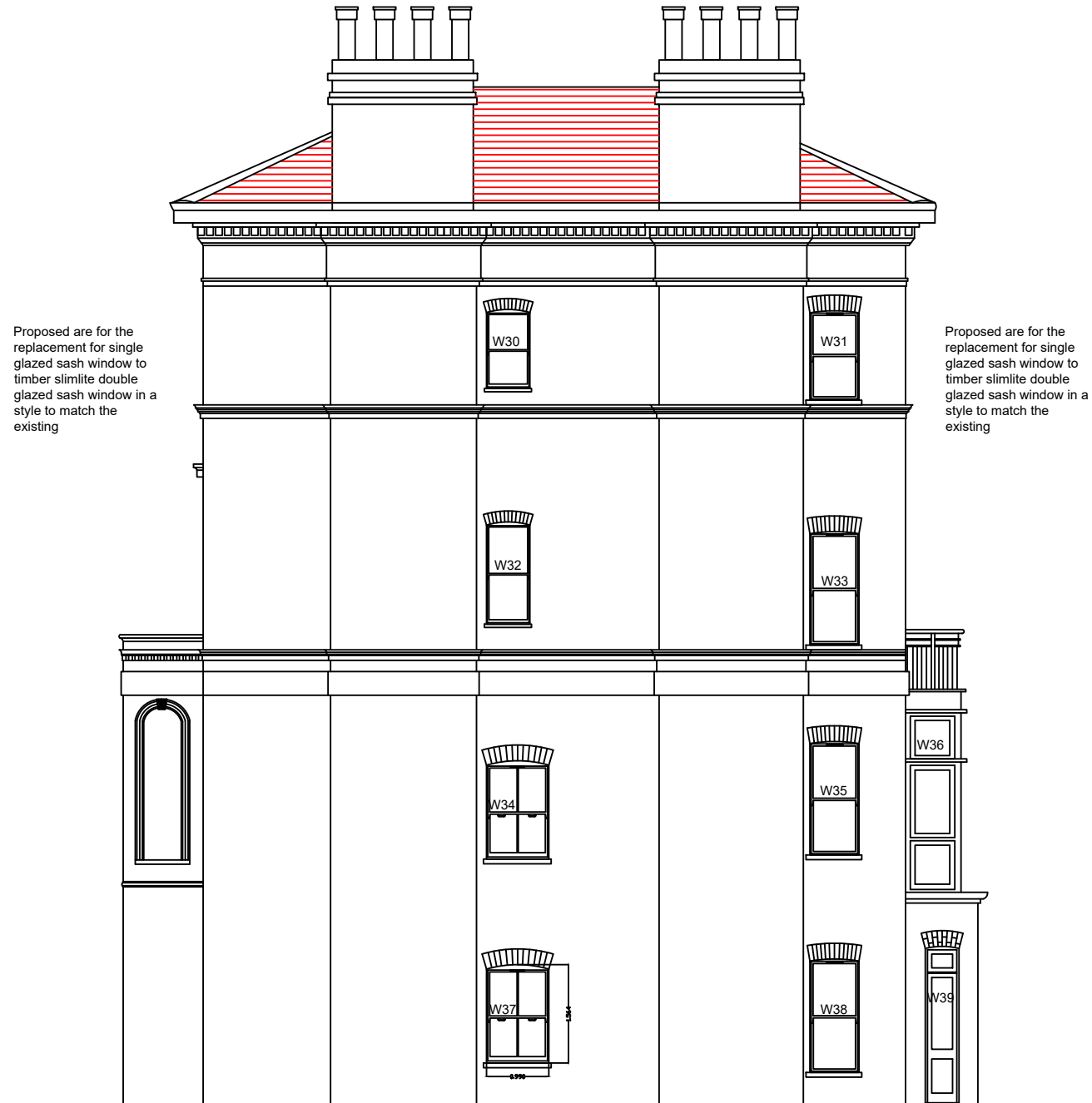
LEFT SIDE ELEVATION (Proposed)
