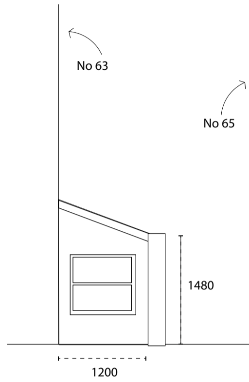
1:50 (@A3): Proposed Extension Elevation
