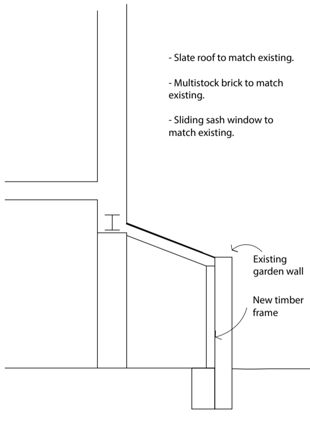
1:50 (@A3) : Section Through Proposed Extension
