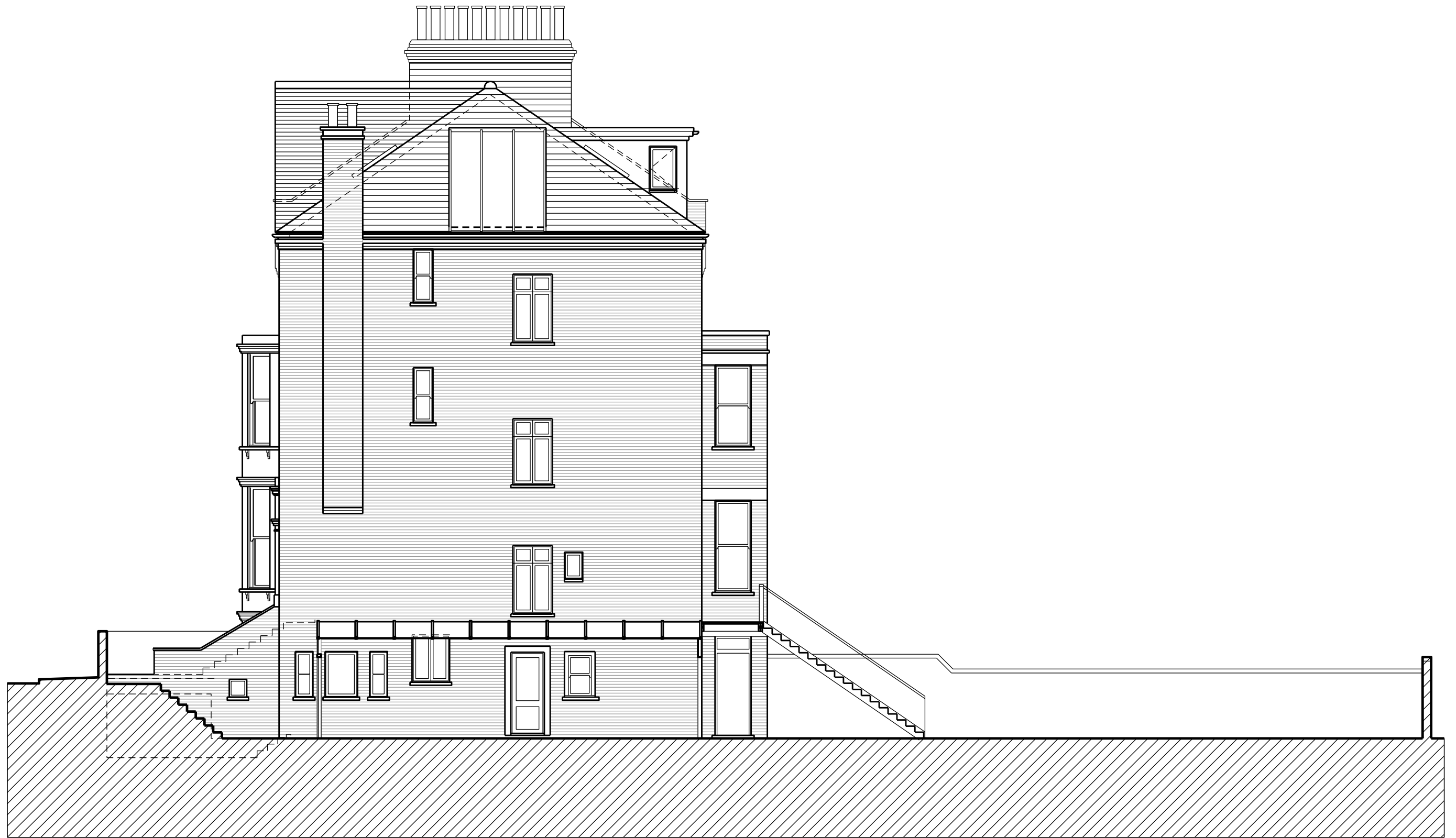
01 Existing Side (SE) Elevation Scale 1:100
