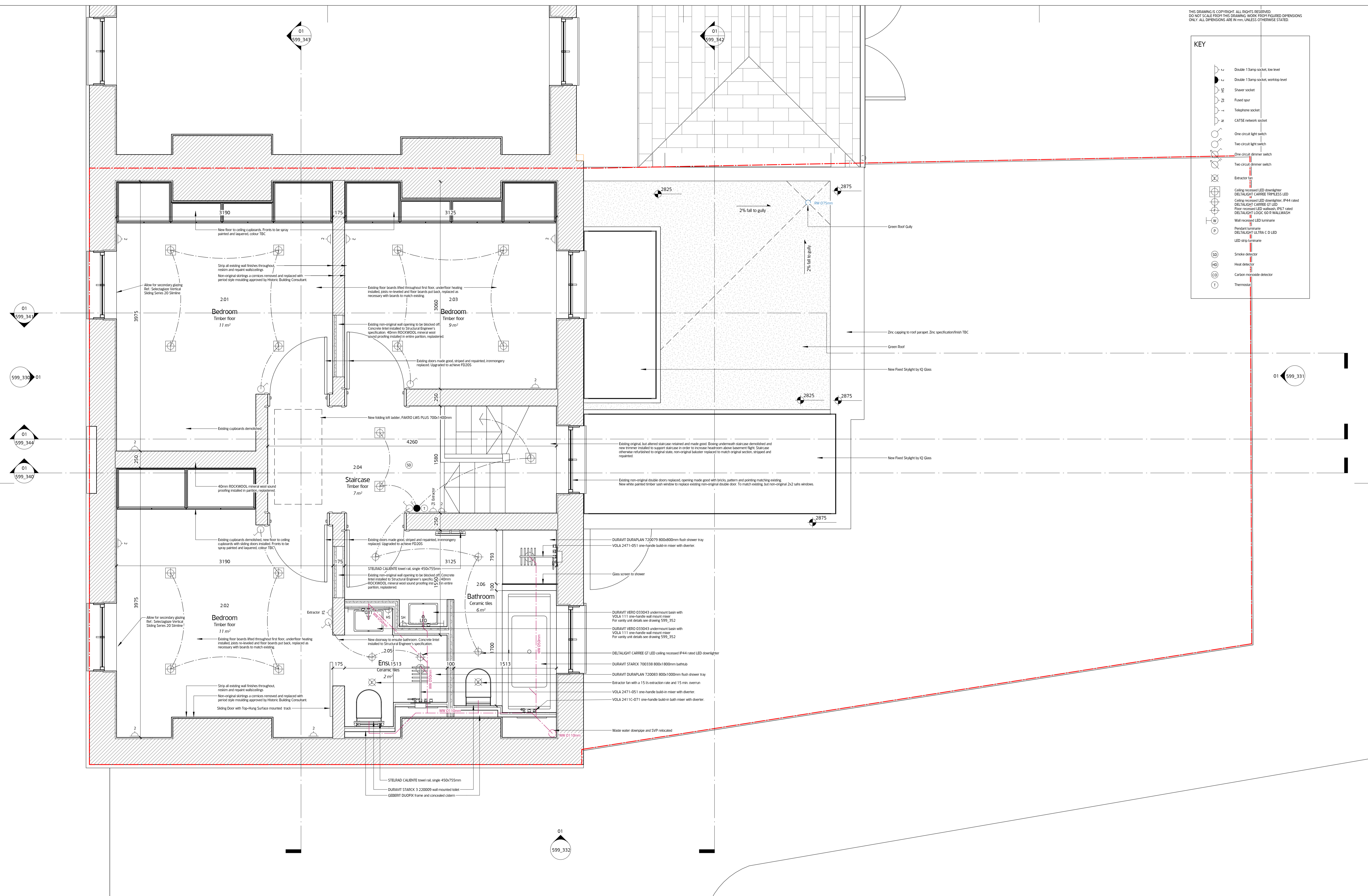
01 Proposed First Floor Plan 1:25
