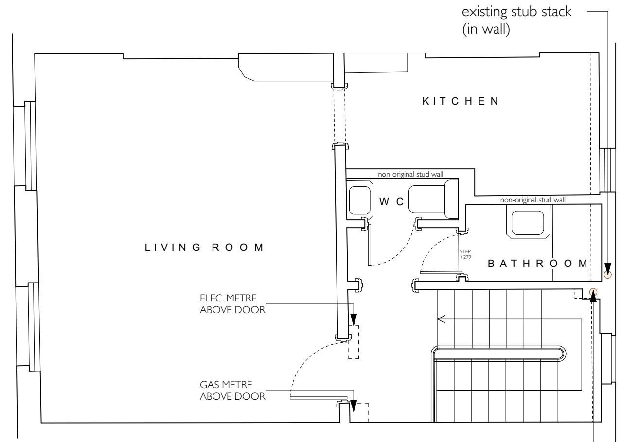
EXISTING THIRD FLOOR PLAN- SCALE 1:50
