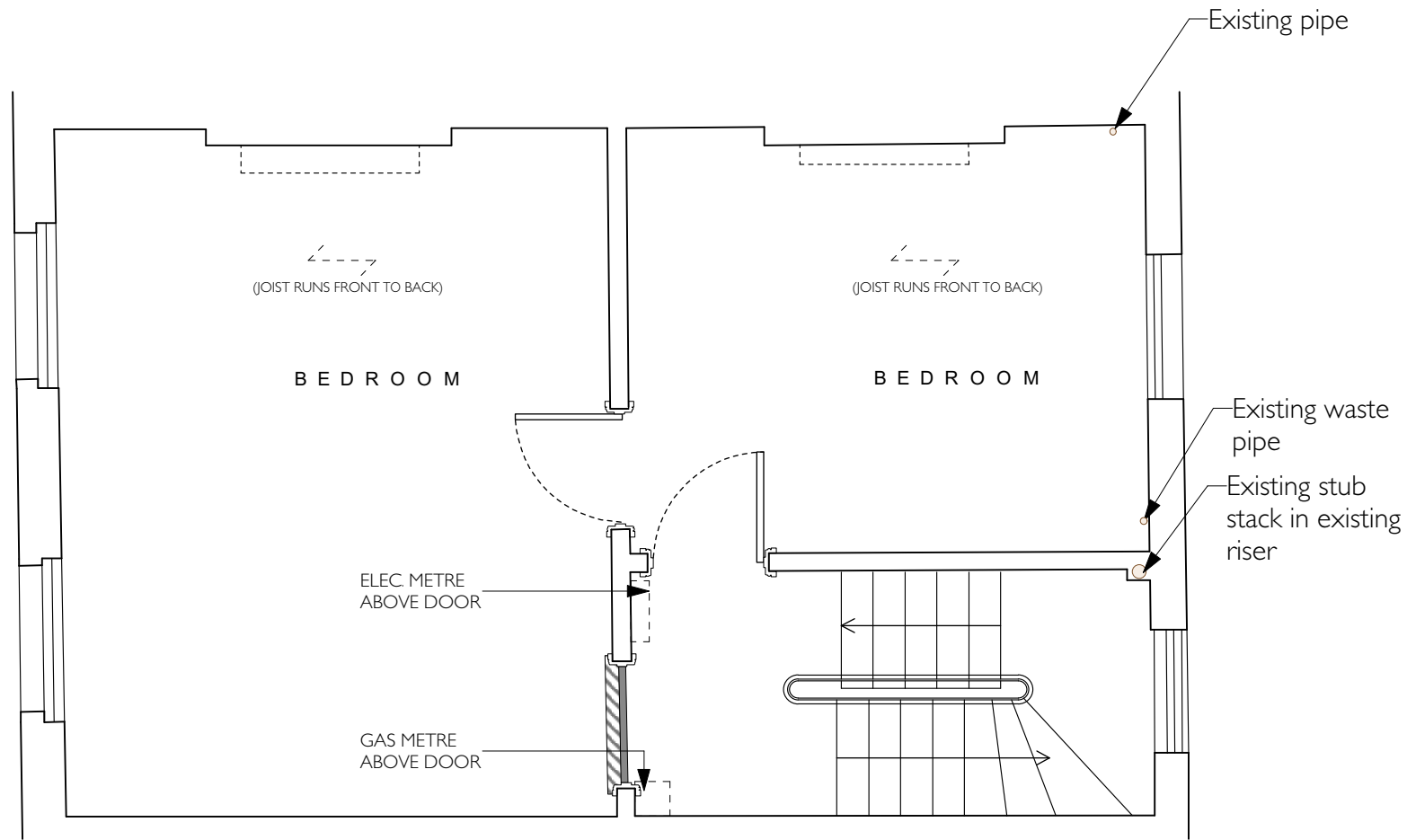
EXISTING SECOND FLOOR PLAN- SCALE 1:50
