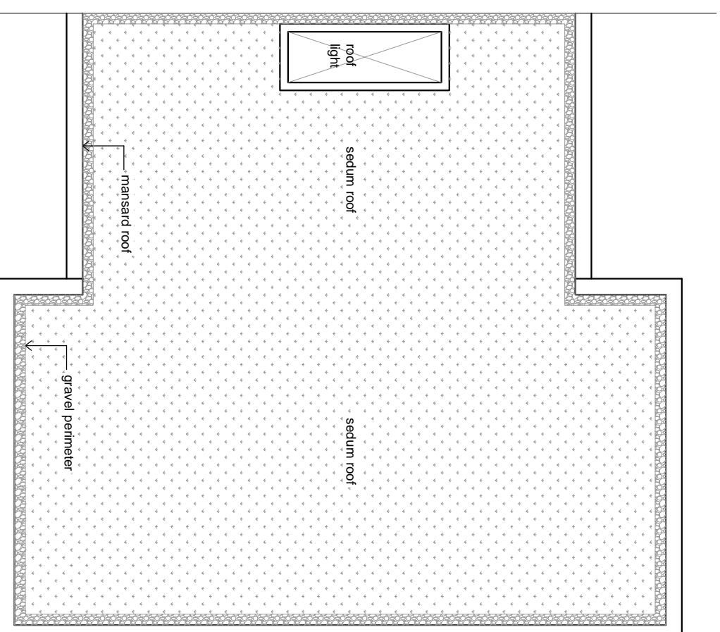
ROOF
