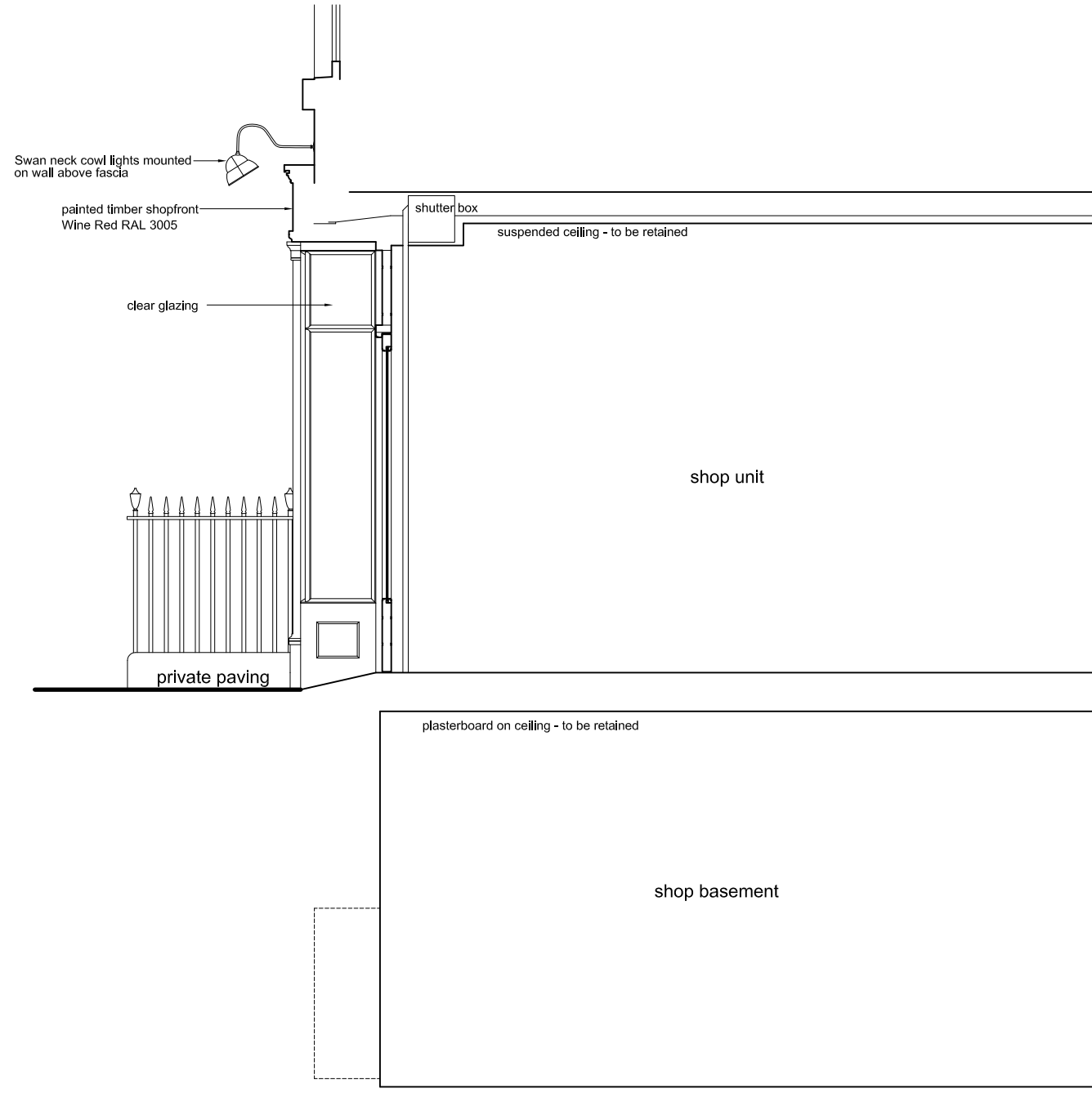
SECTION 0 1m
