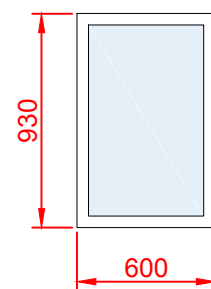
R3 Bed 3 Casement
