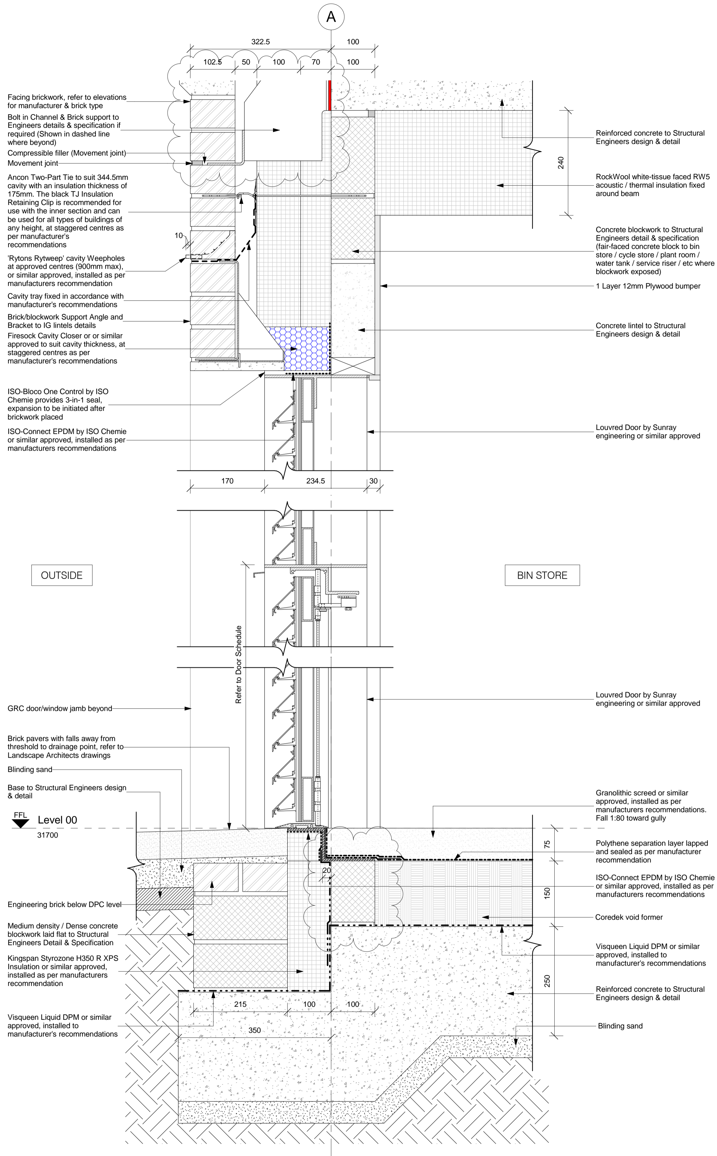
1 Typical Louvre Door Head and Cill Detail 16.04 1:5
