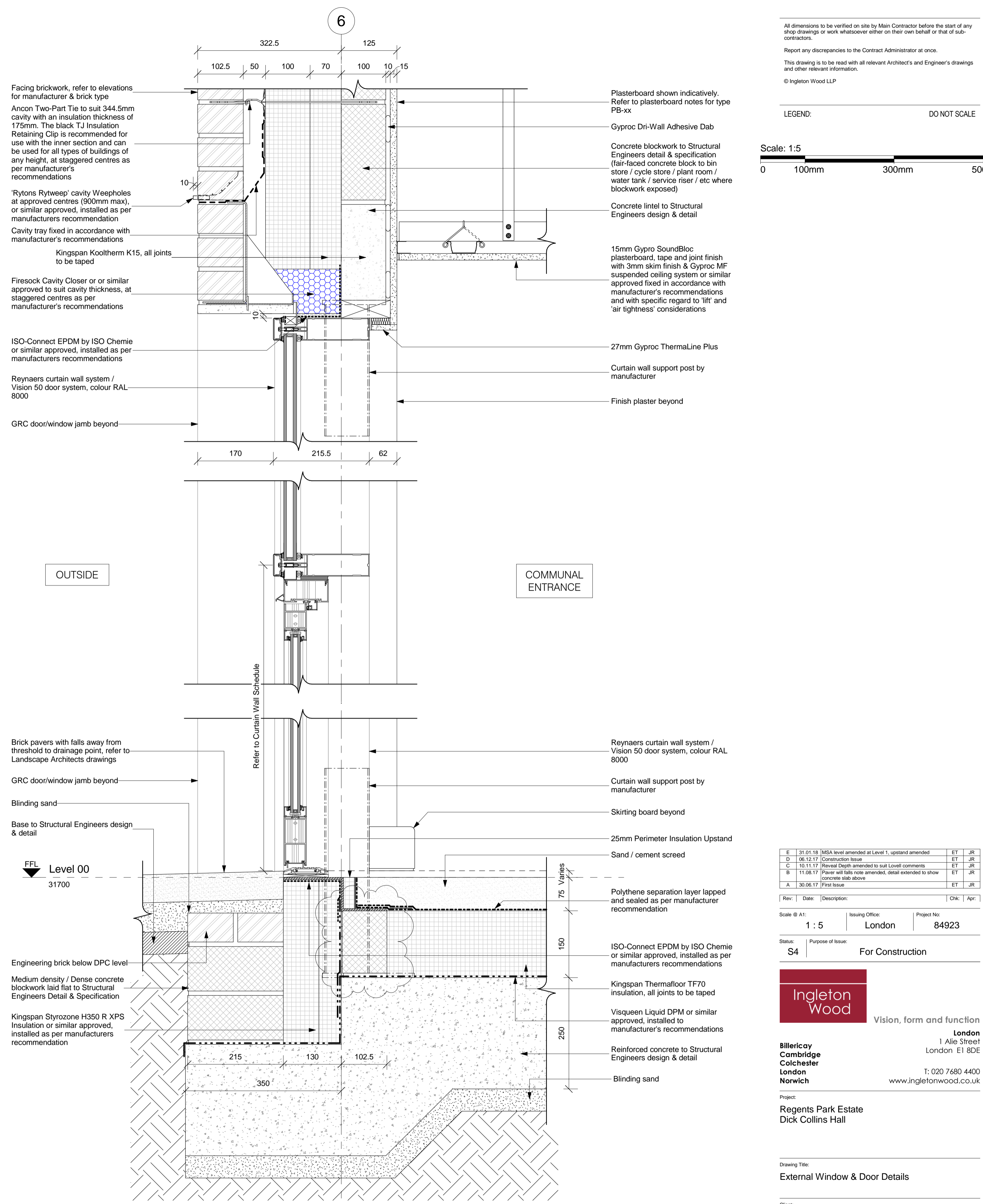
2 Typical Curtain Wall Door Head and Cill Detail 16.04 1:5
