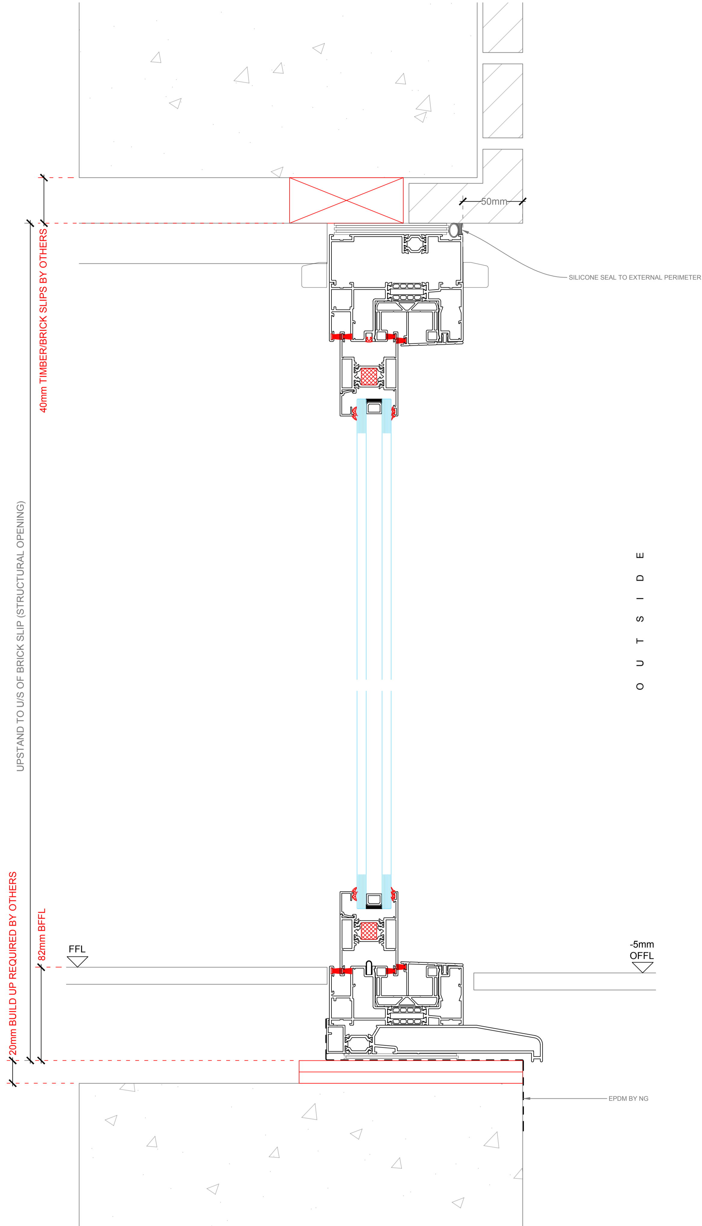
SECTION THROUGH DOORSET : A 1:2 @ A1
