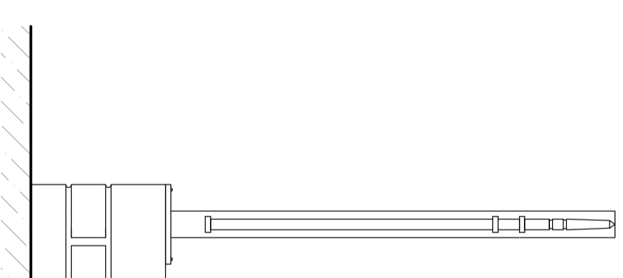
Railing Detail (1:10)
