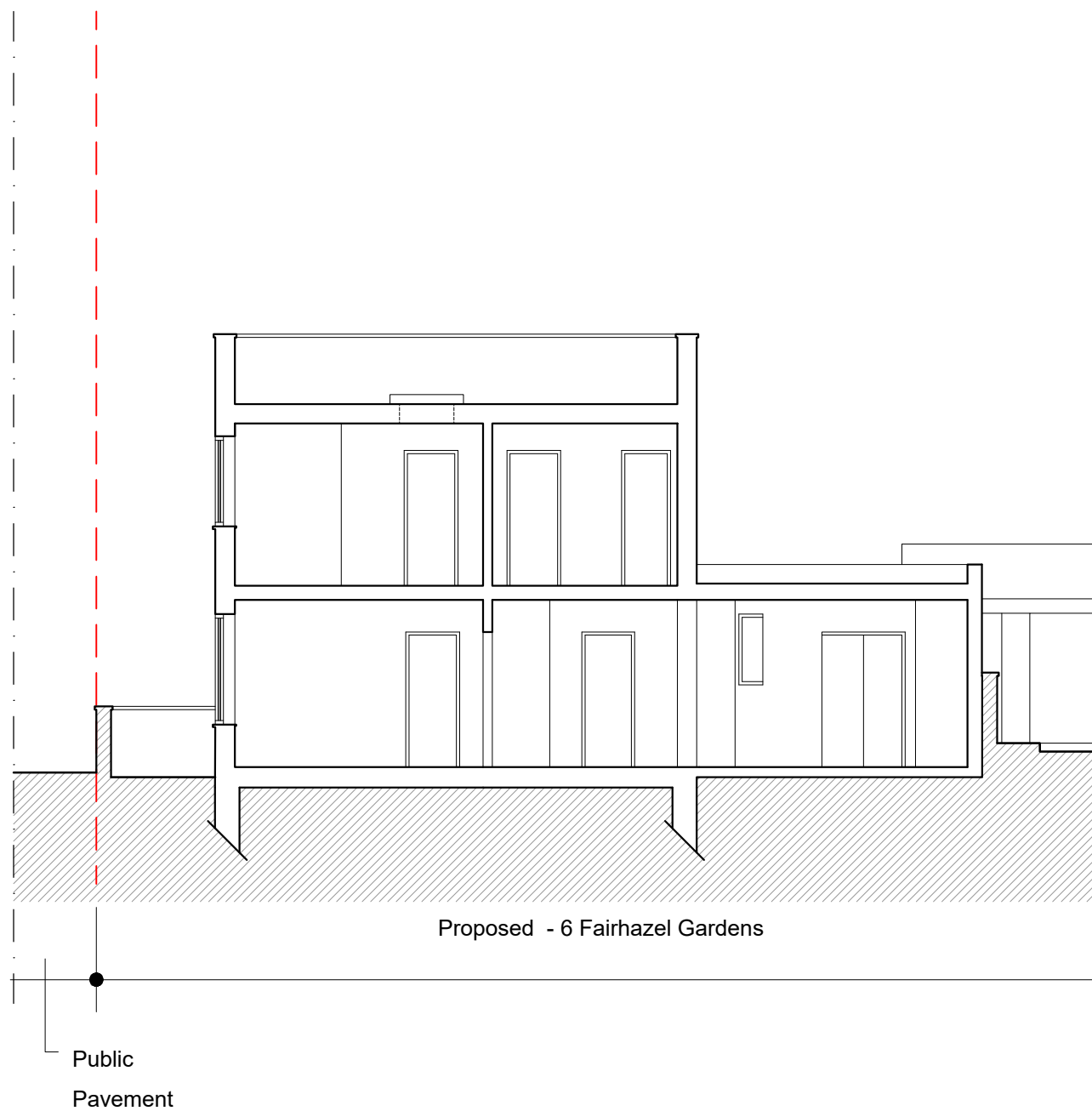
Section AA'
