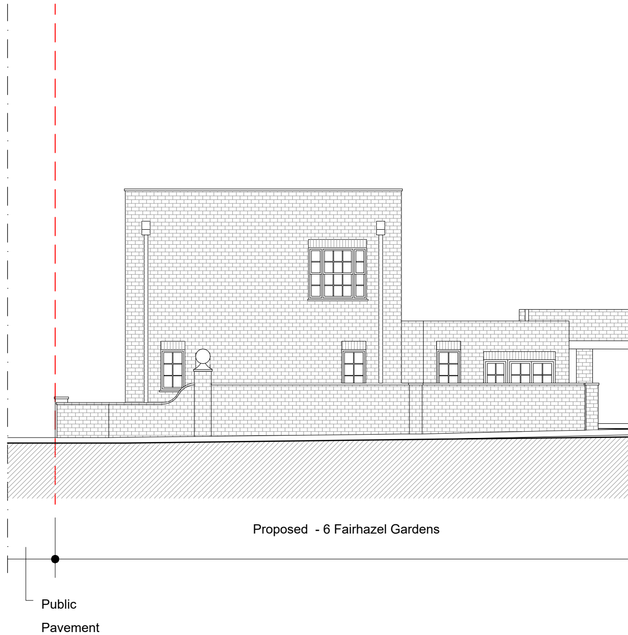
Side Elevation 1
