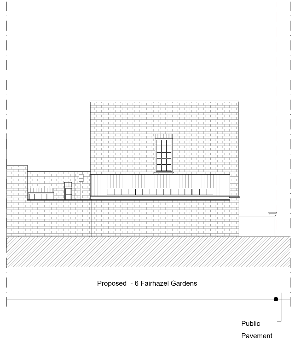
Side Elevation 2
