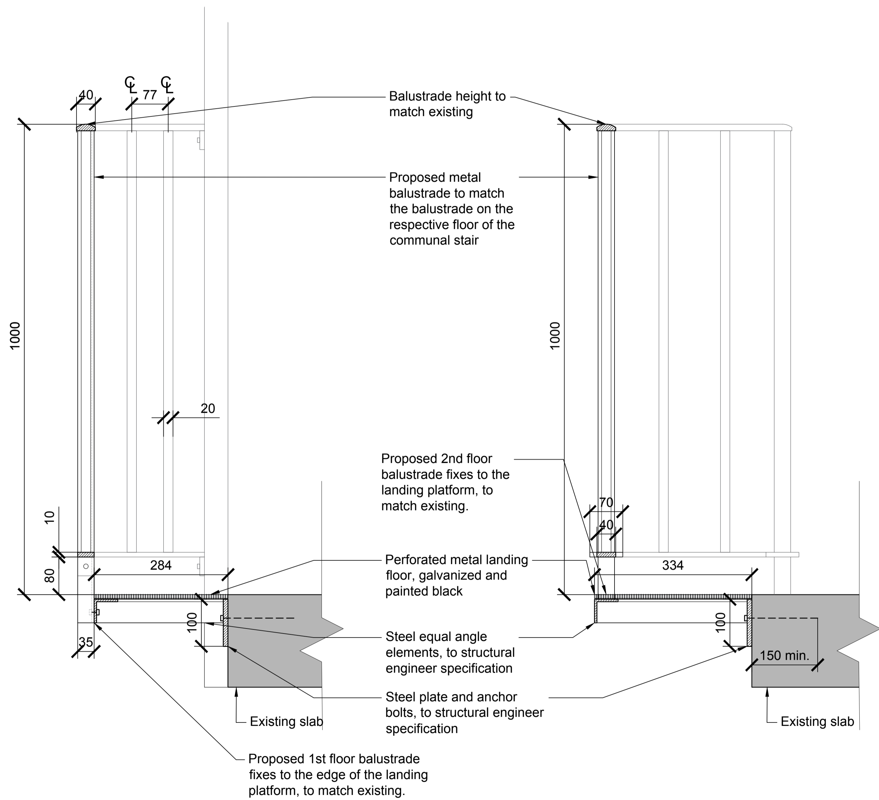
2 - FIRST FLOOR LANDING PLATFORM: BALUSTRADE DETAIL 1:5
