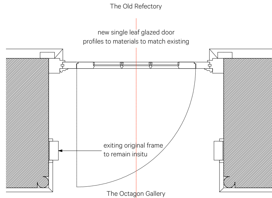
Proposed FD-30 entrance door plan high level 1:10
