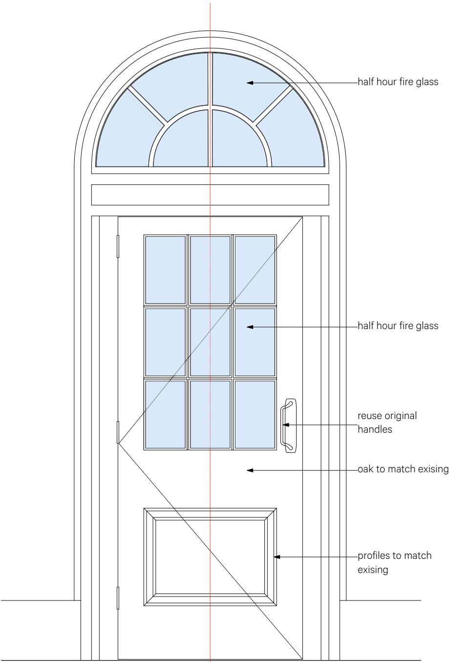
Proposed FD-30 door elevation from The Octagon Gallery 1:10
