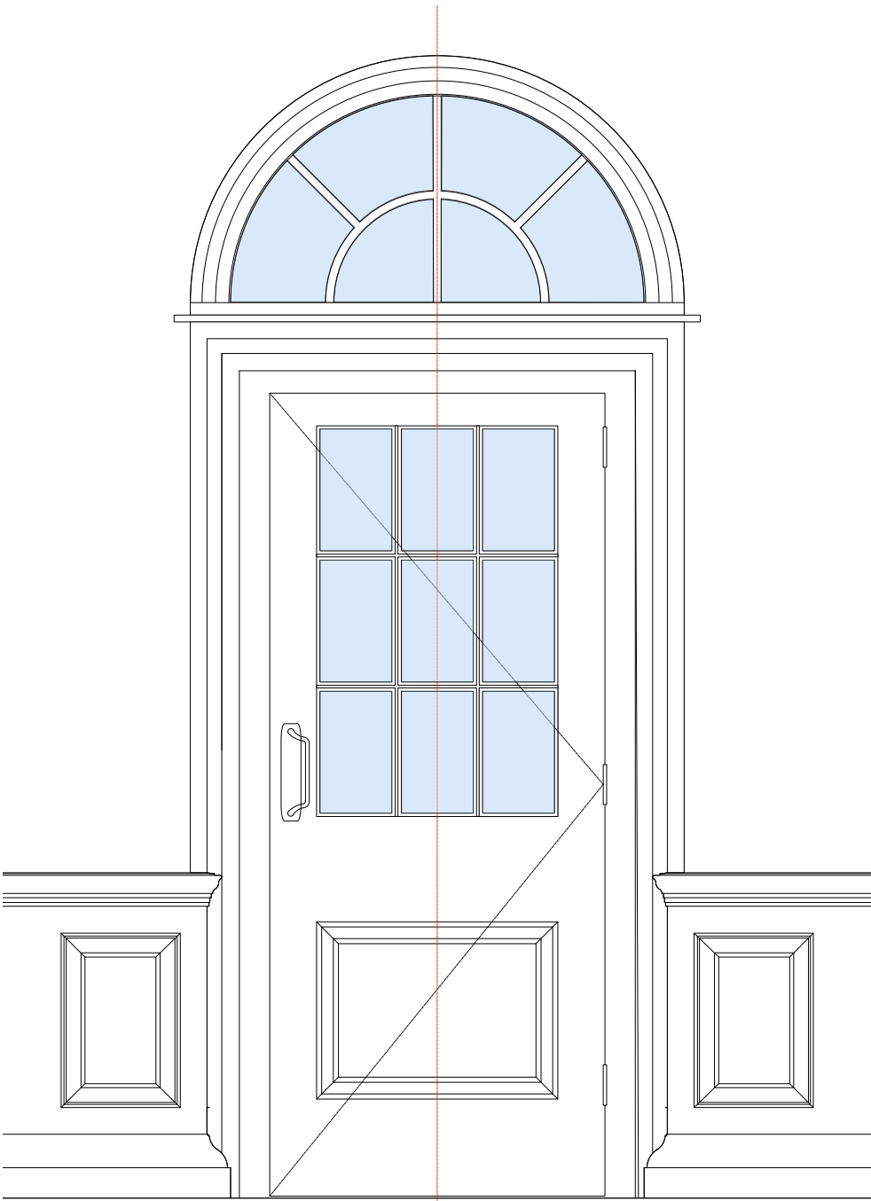
Proposed FD-30 door elevation from The Old Refectory 1:10
