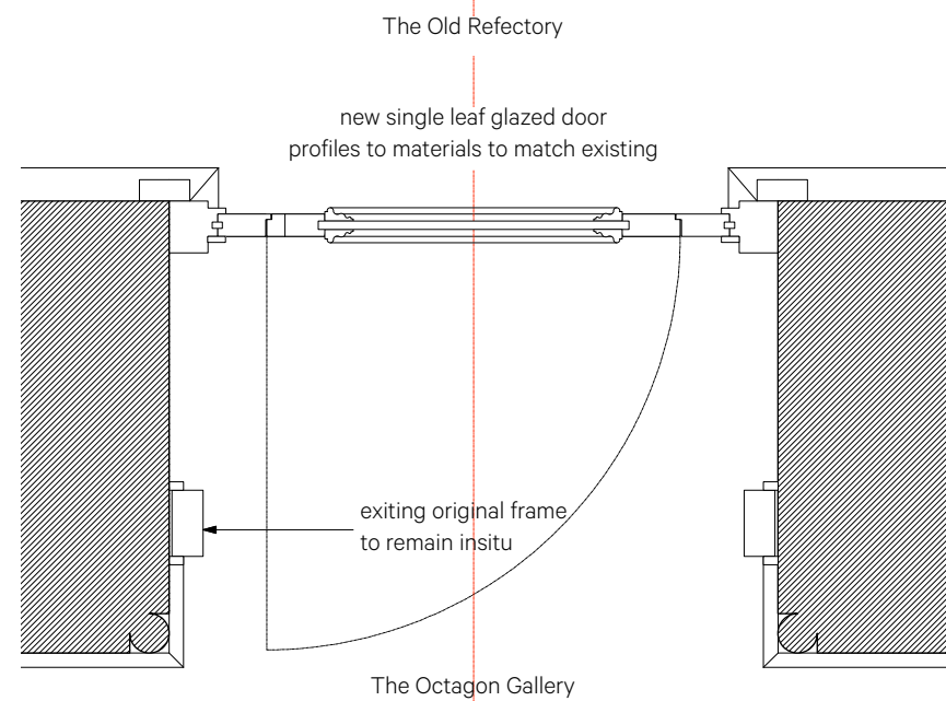
Proposed FD-30 entrance door plan high level 1:10
