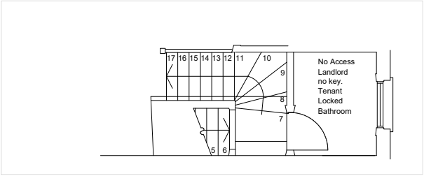
Existing Second & Third Mezzanine Level 1:100
