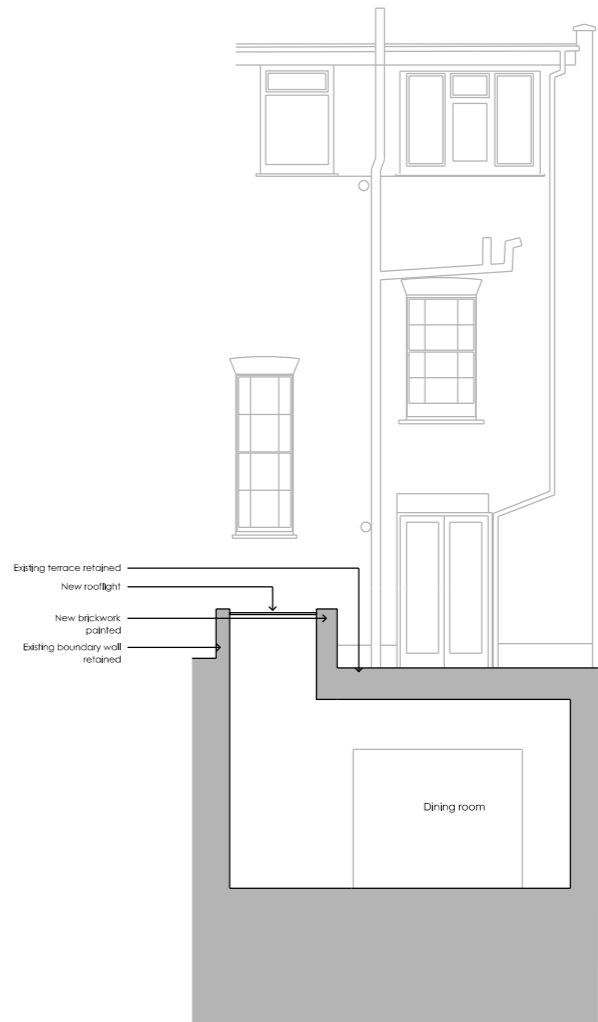
Proposed Section BB
