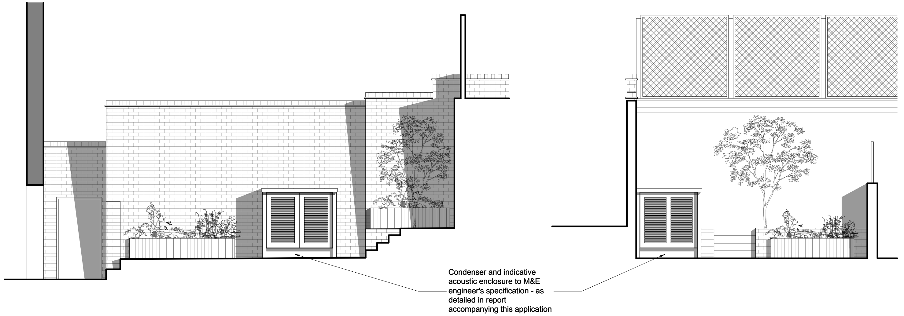
Proposed front and side elevation of condenser and acoustic enclosure
