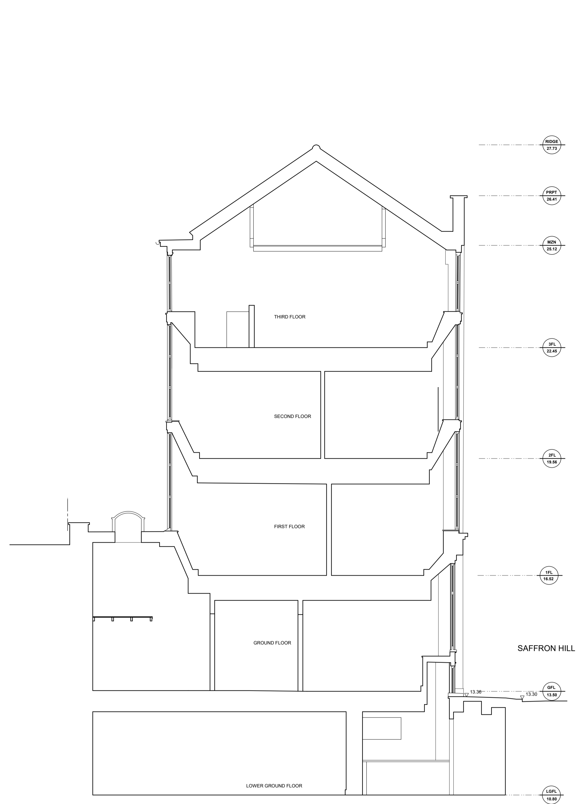
SECTION A - A (A.O.D 10.00m)
