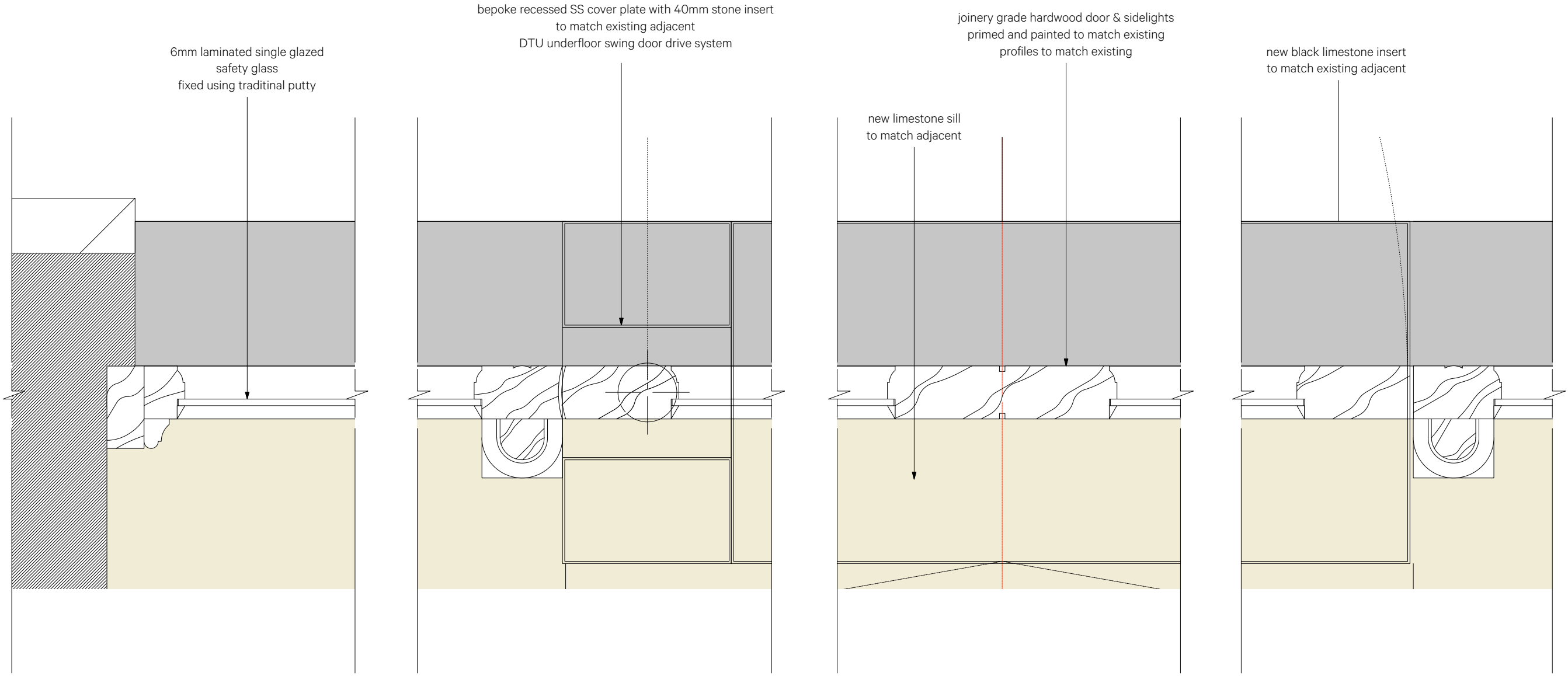
AUTOMATED DOORS - JAMB DETAIL SCALE 1:2 @ A1 Half actual size
