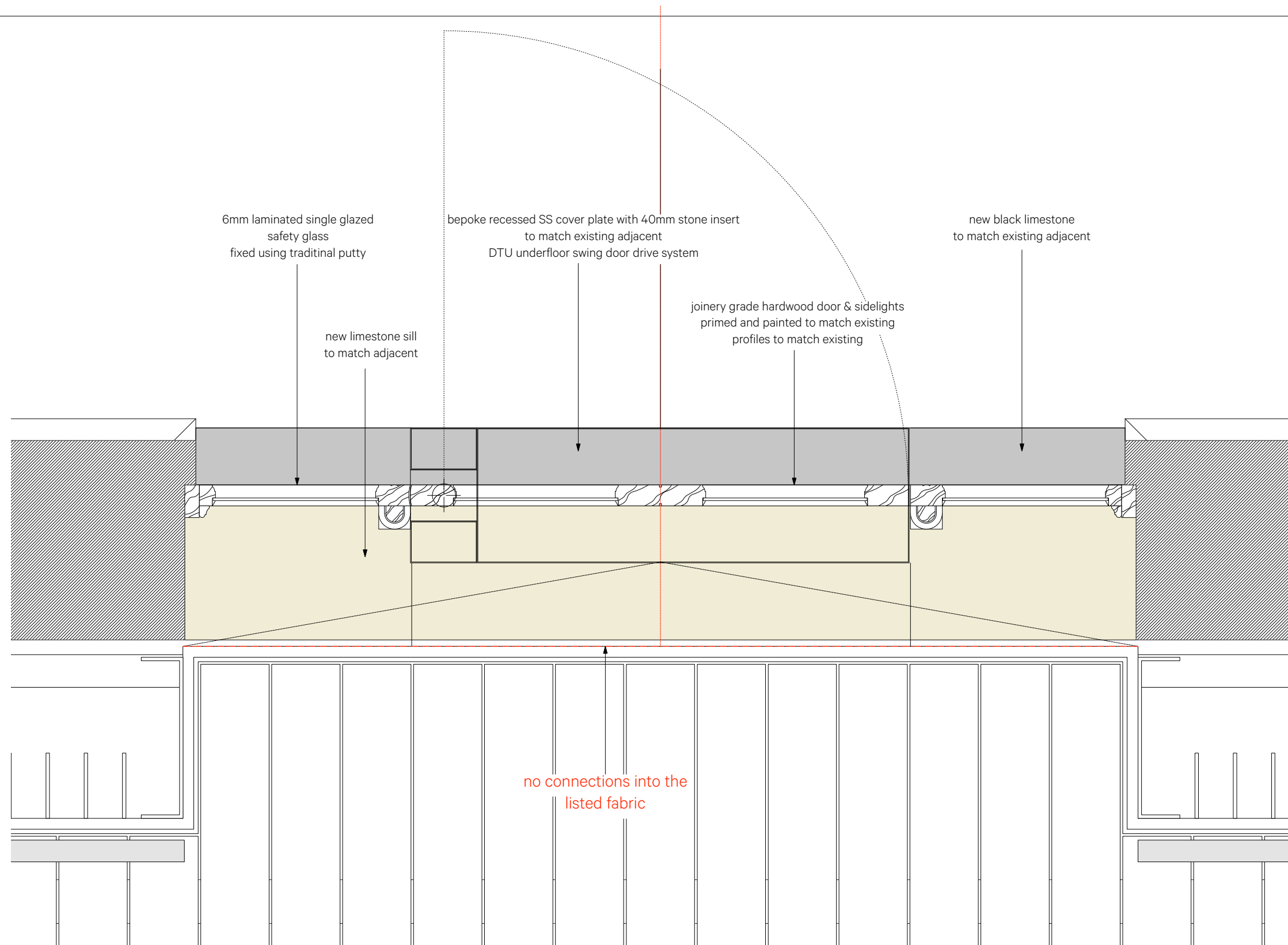
AUTOMATED DOORS - JAMB DETAIL SCALE 1:5 @ A1
