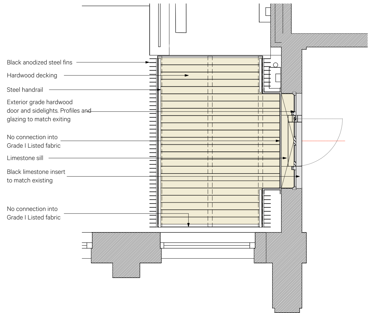
Upper ground floor plan
