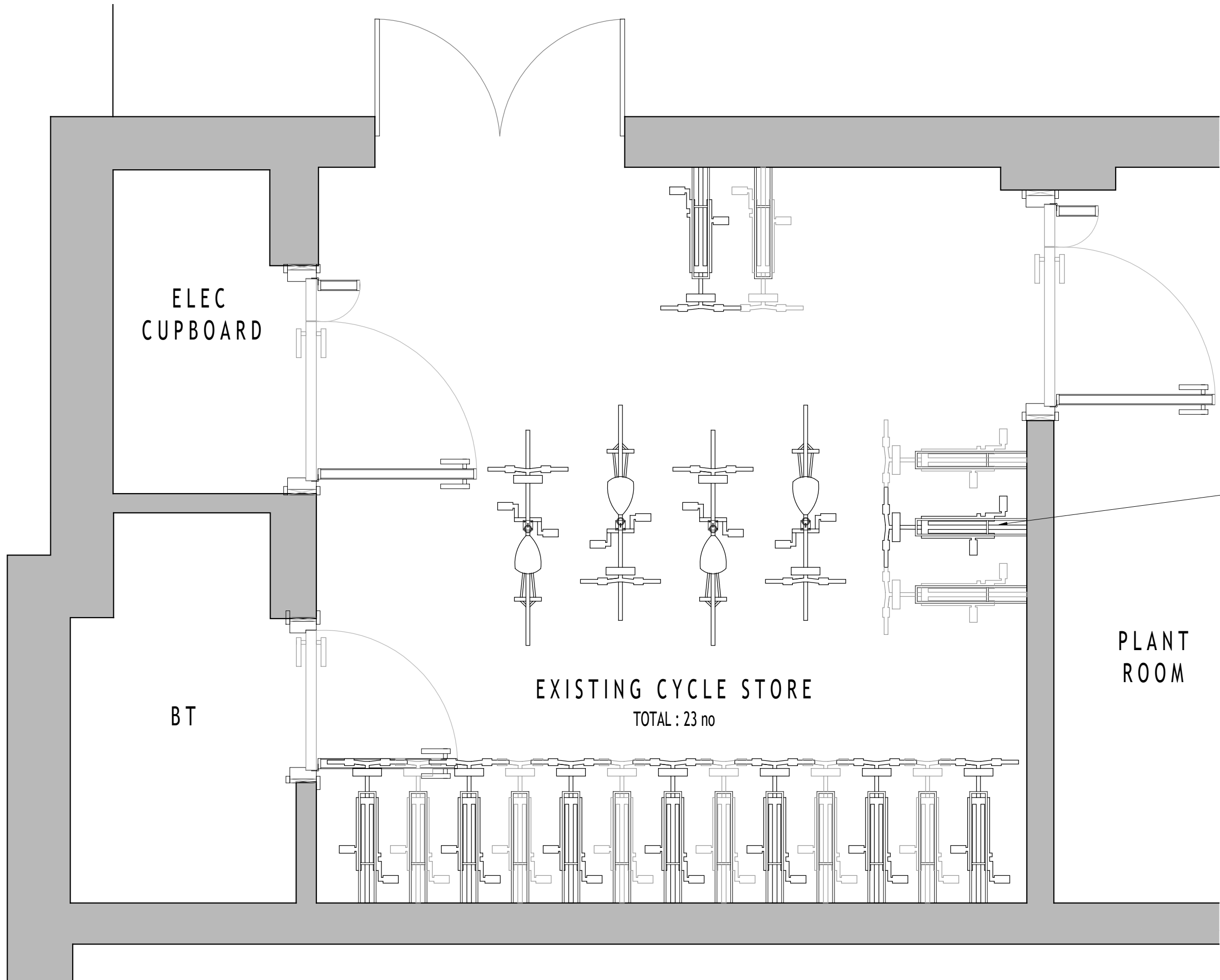
Existing Cycle Store 1:20@A3
