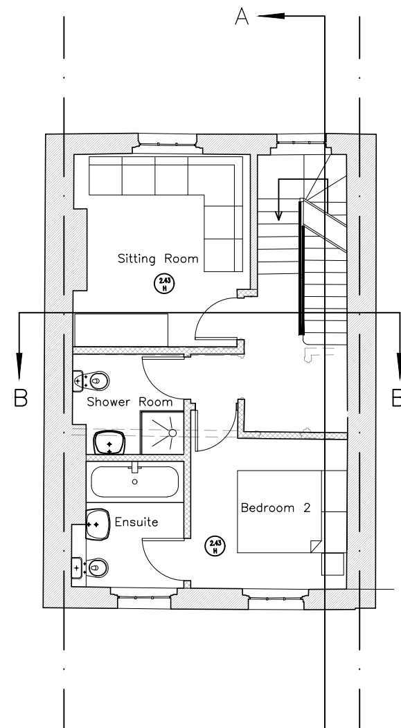
Proposed Second Floor SCALE 1:100
