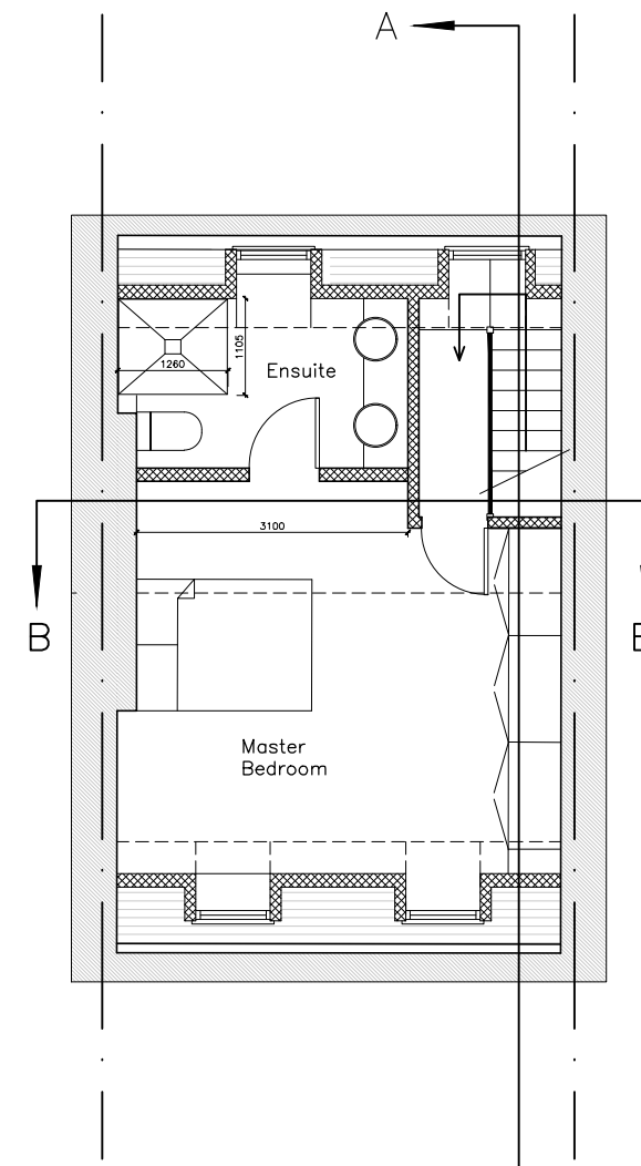
Proposed Third Floor SCALE 1:100
