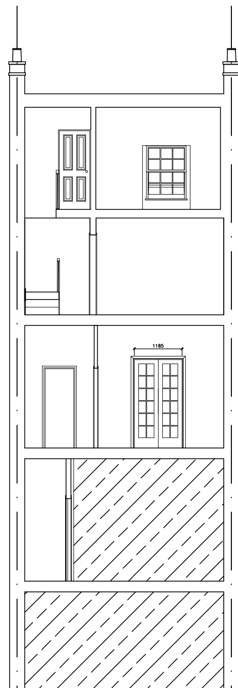
Proposed Section B-B SCALE 1:100
