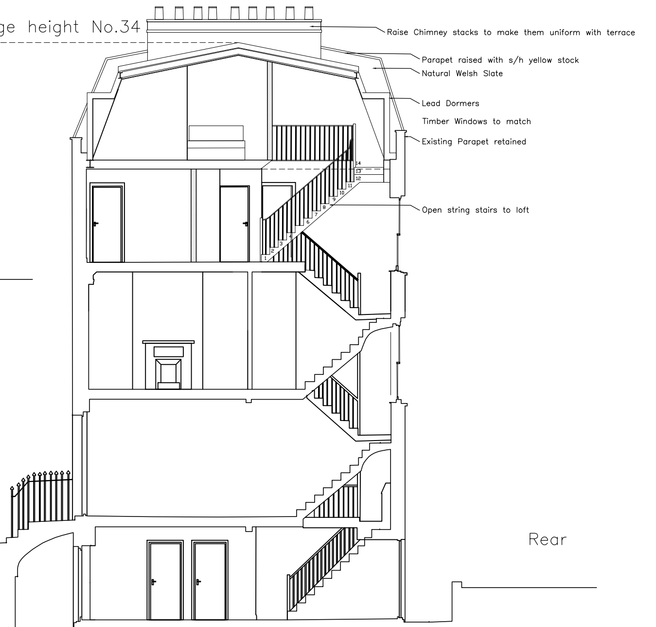
Proposed Section A-A SCALE 1:100
