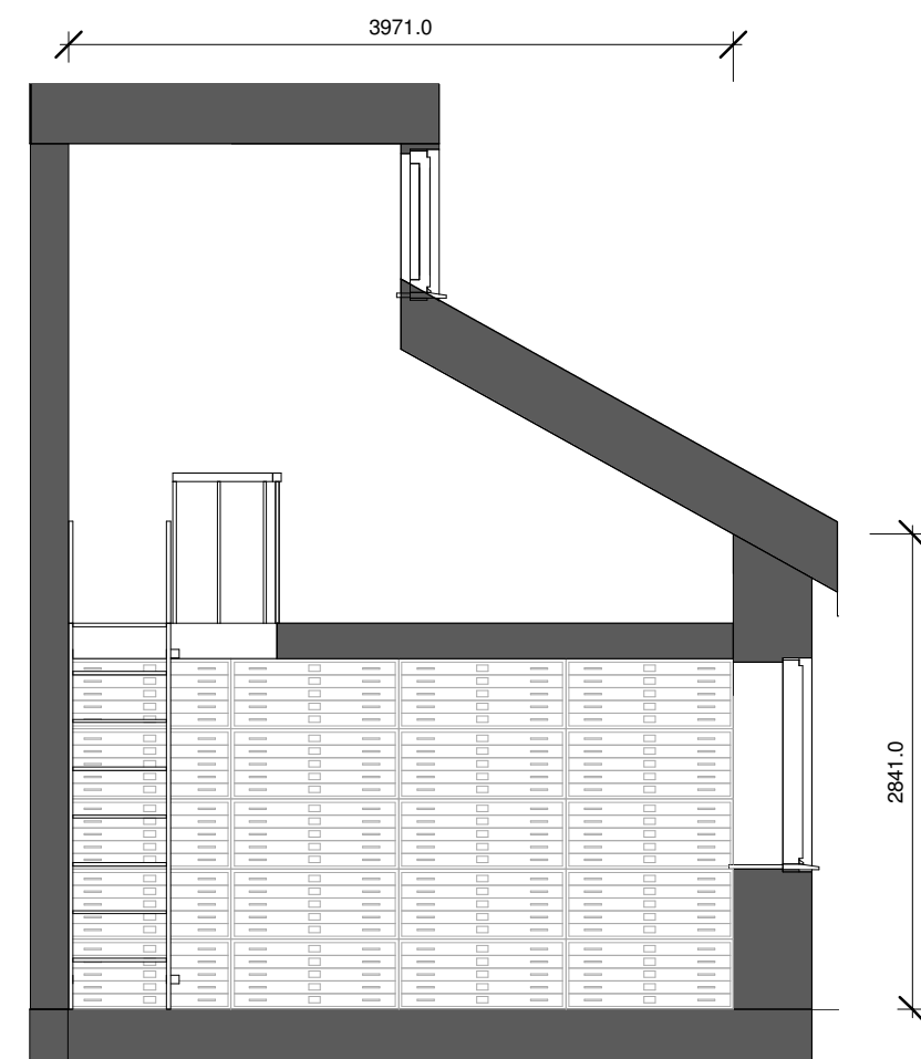
2.5 X18A-Elevation 1 : 50
