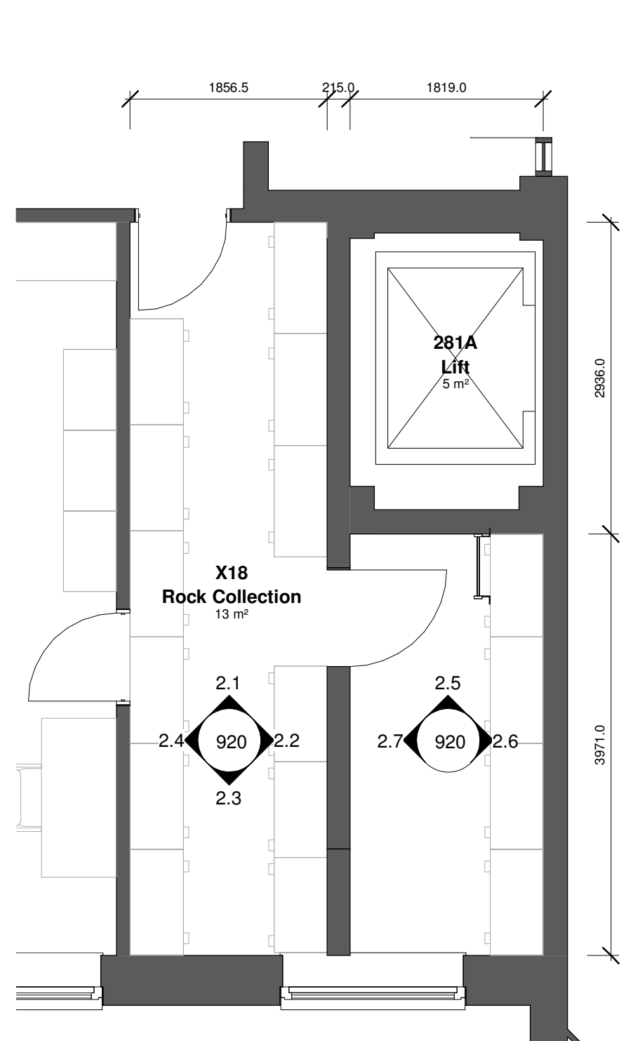
1.1 Existing Rock Collection&Store Plan 1 : 50
