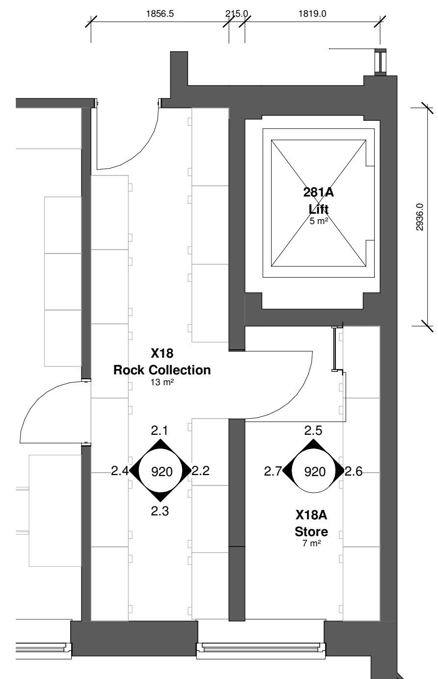
1.2 Existing Rock Collection&Store Mezzanine Plan 1 : 50
