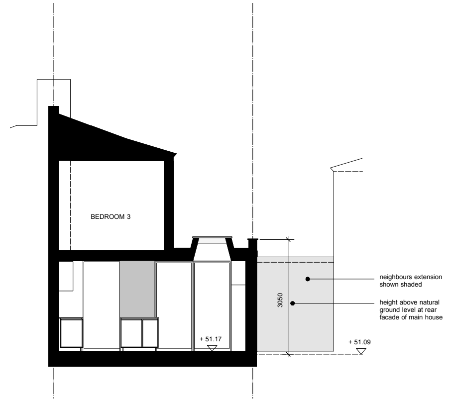
2 cross section B
