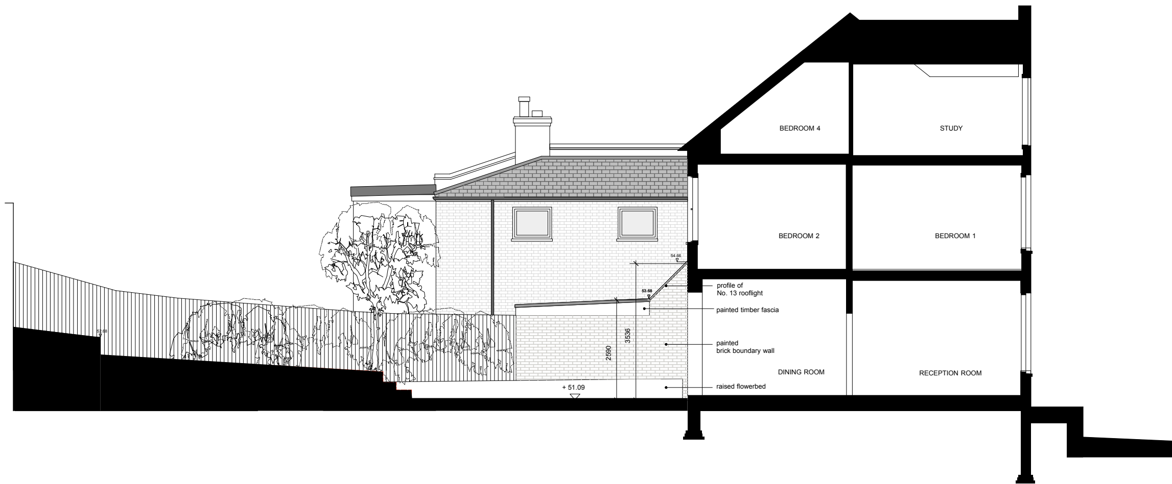
1 existing long section C
