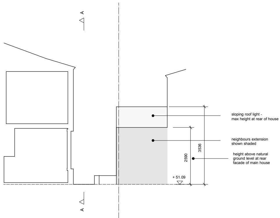
2 existing cross section B
