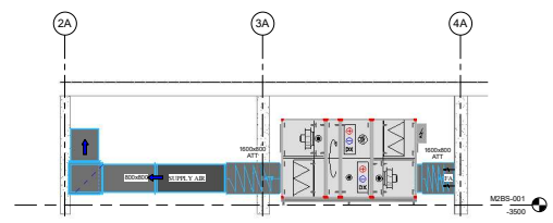
2 M2BS-005-Section 1 North 1:50
