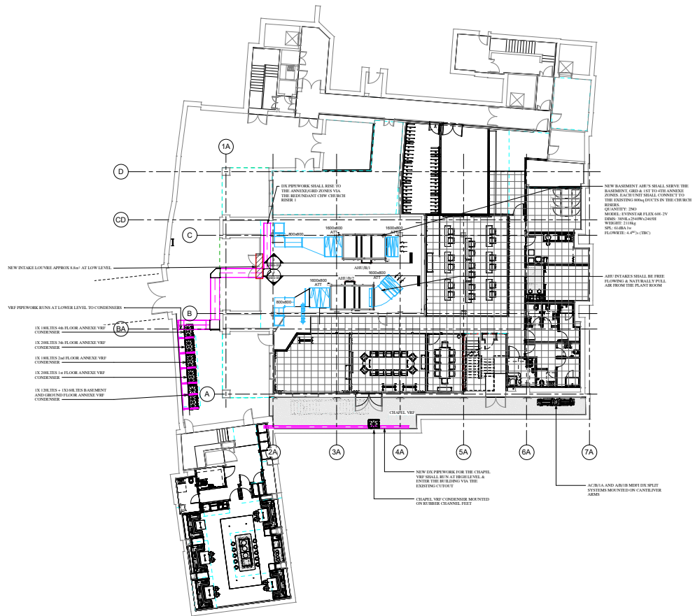
1 M2BS-005-Basement AHU 1:100
