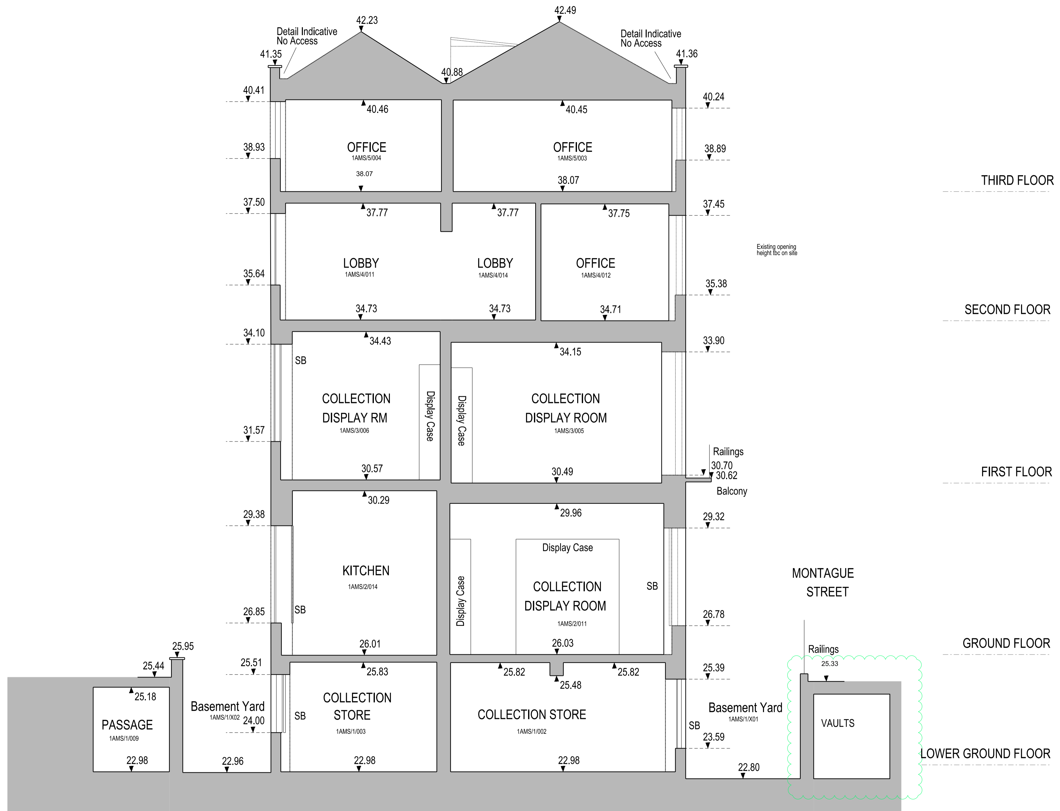
SECTION BB' 20.00m Above Ordnance Datum
