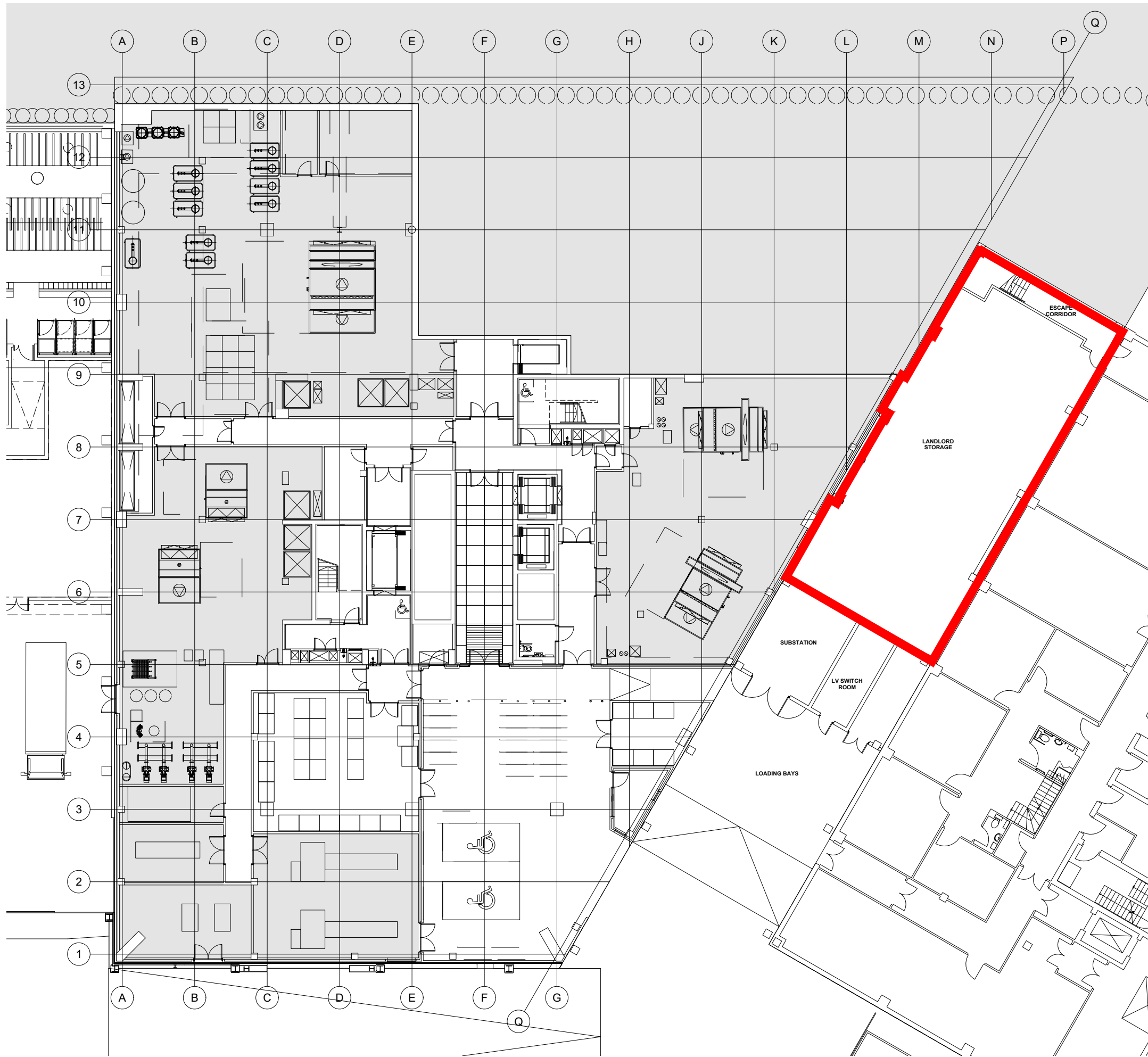
1:250@A3 EXISTING LOWER BASEMENT PLAN
