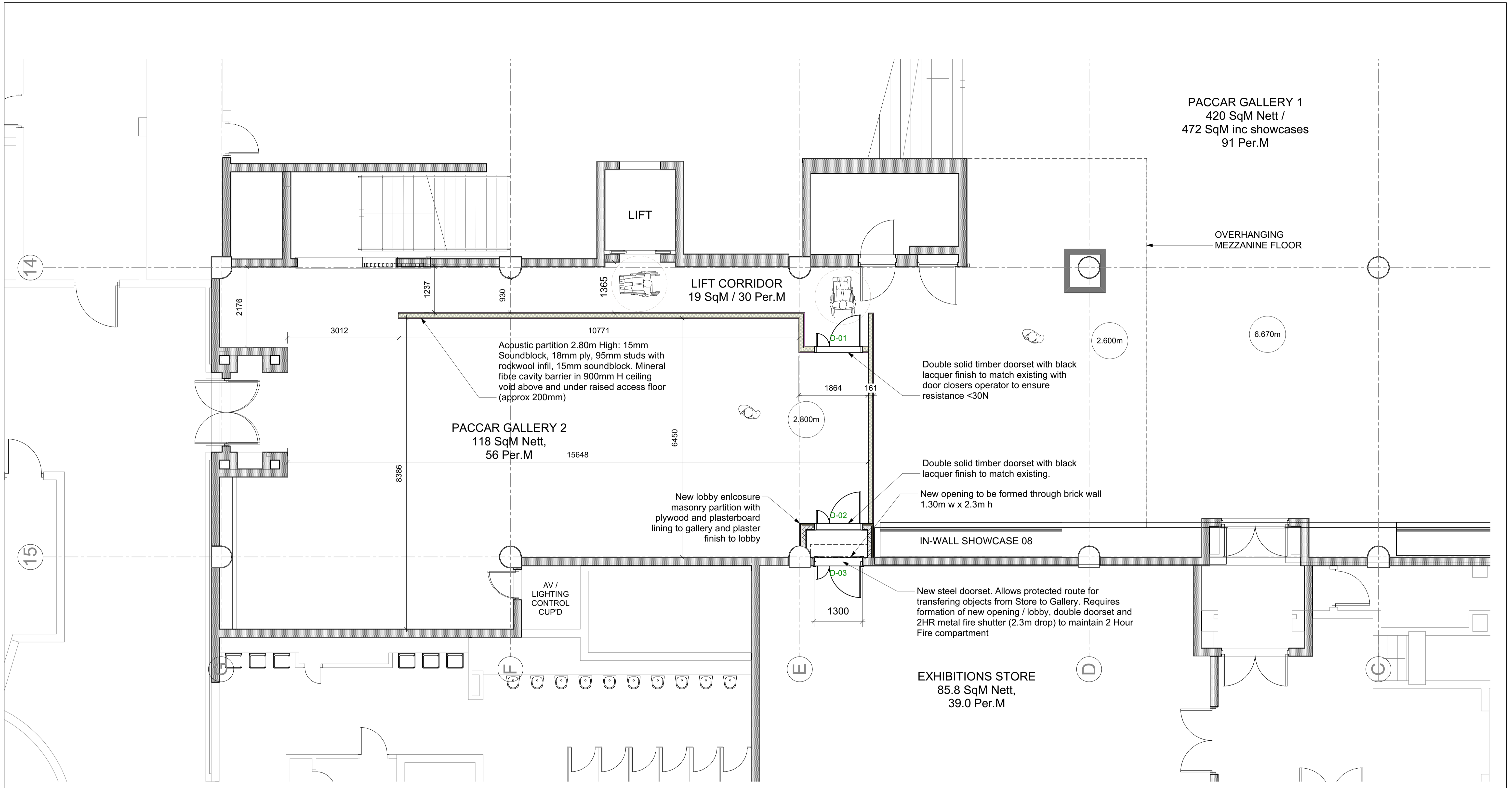
2 LOWER GROUND FLOOR PLAN Scale: 1:50 0 5 10 M
