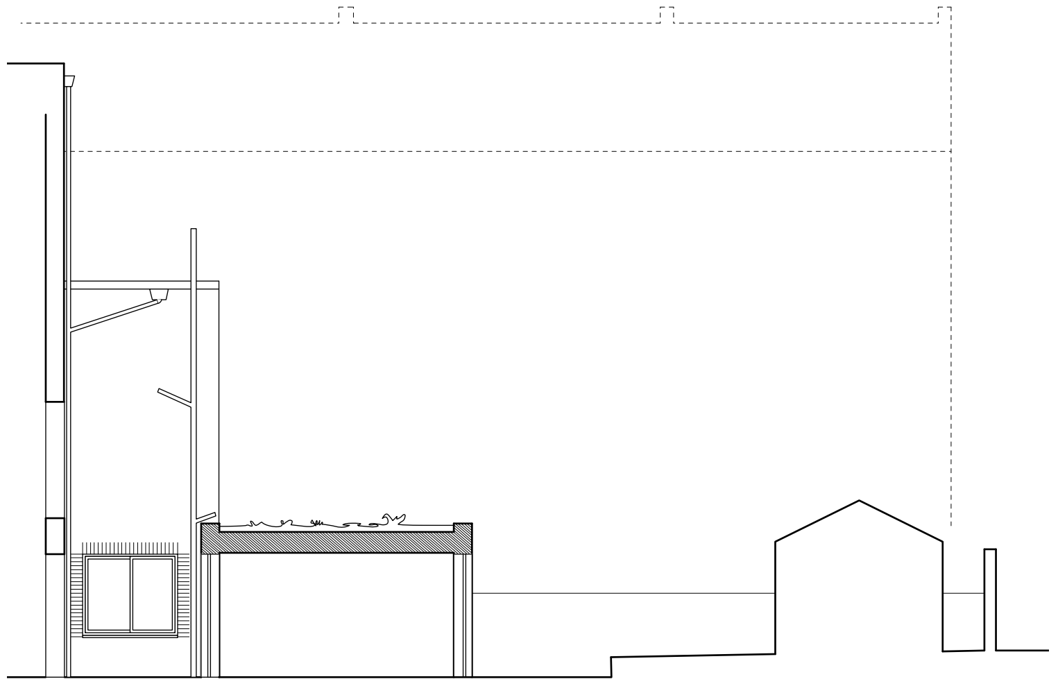
part section aa (through garden of 1 Evangelist Road)
