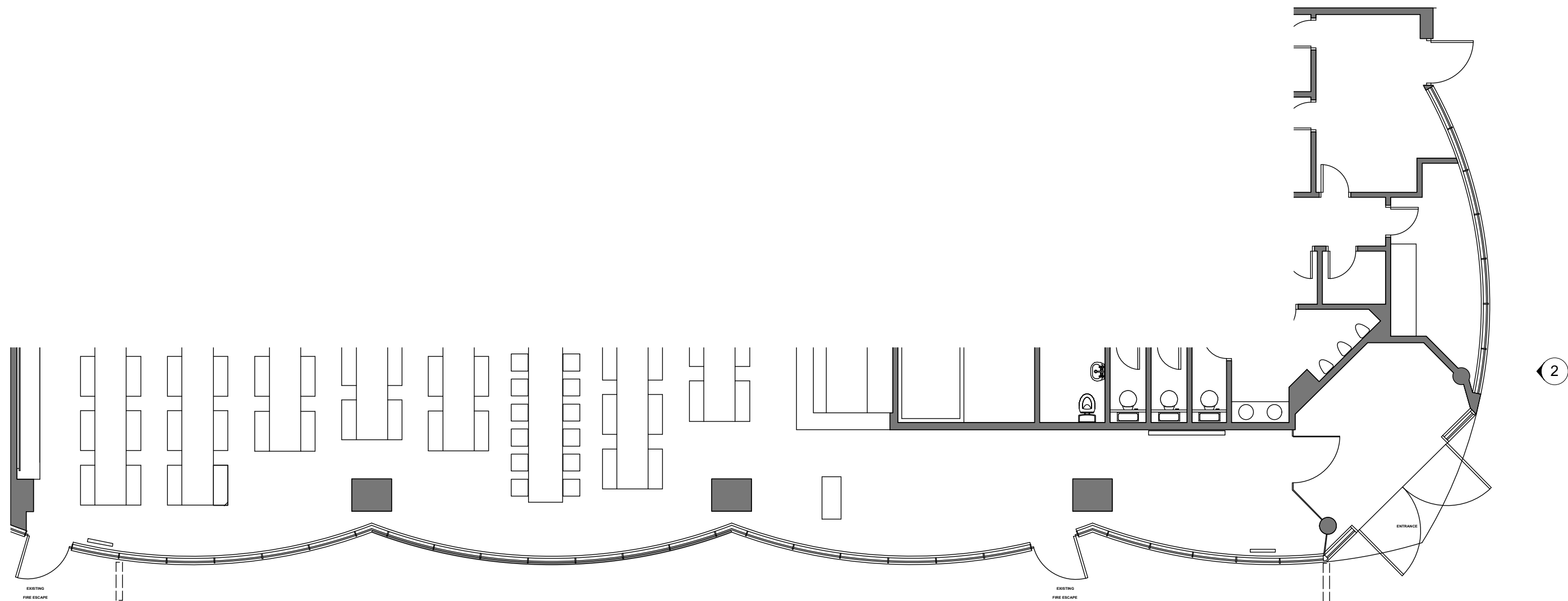
1 Existing Facade Glazing Plan Scale: 1:100
