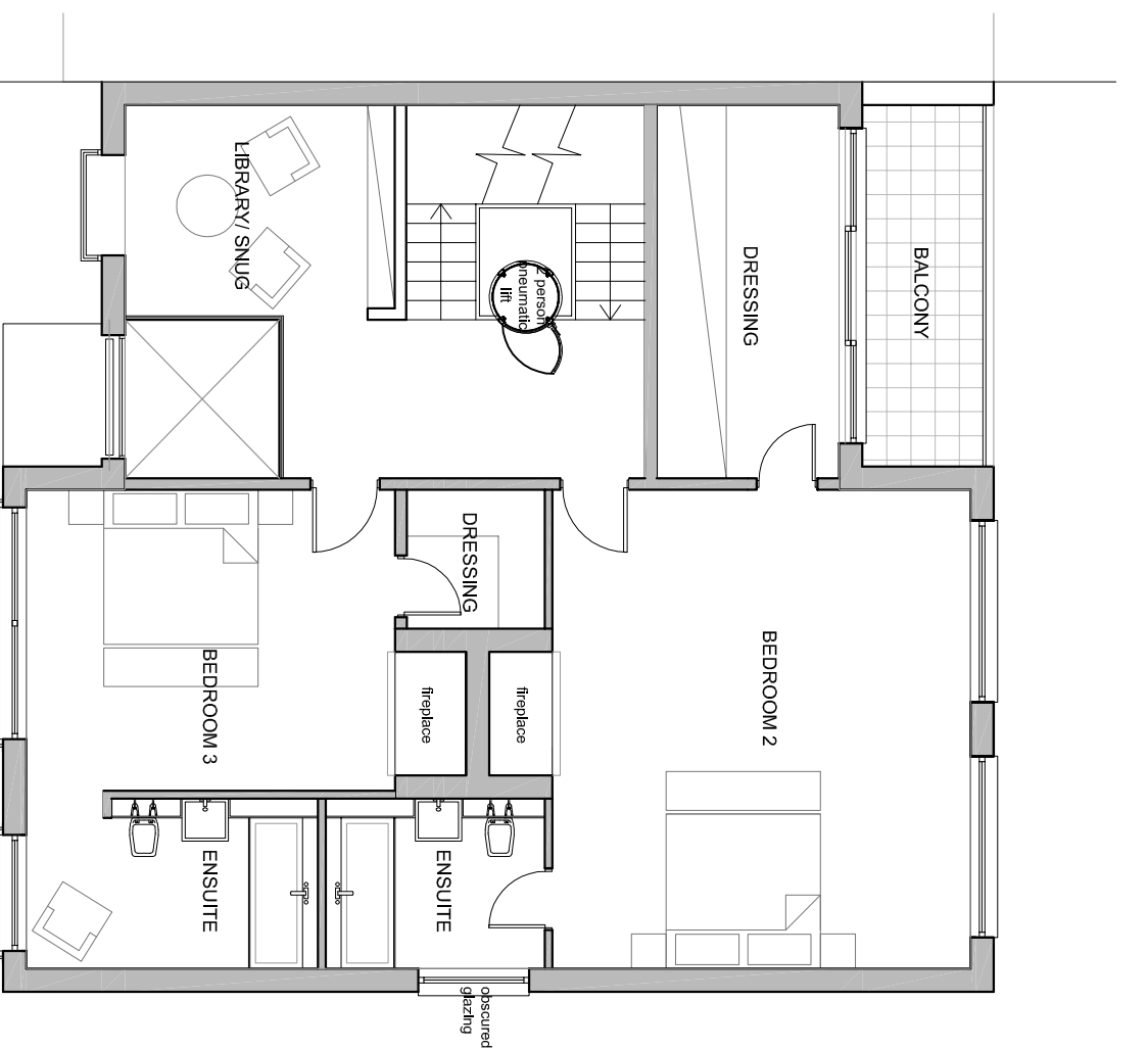
FIRST FLOOR
