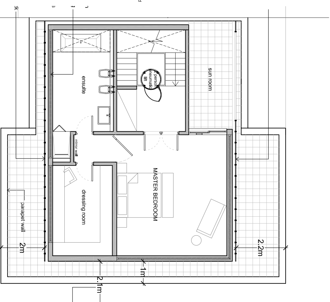
SECOND FLOOR
