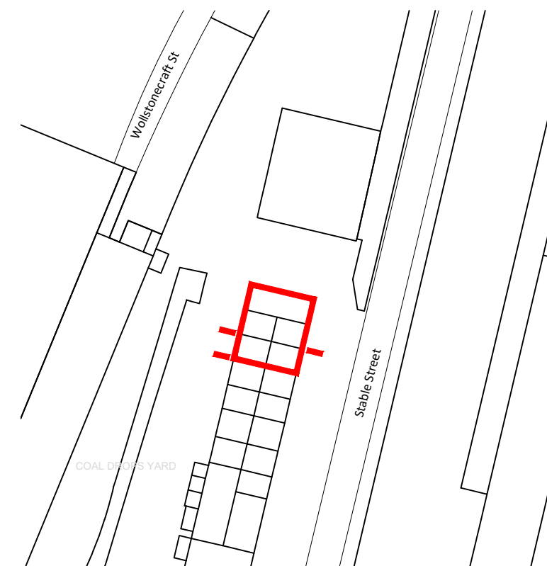
05 LOCATION PLAN 404 1:1250
