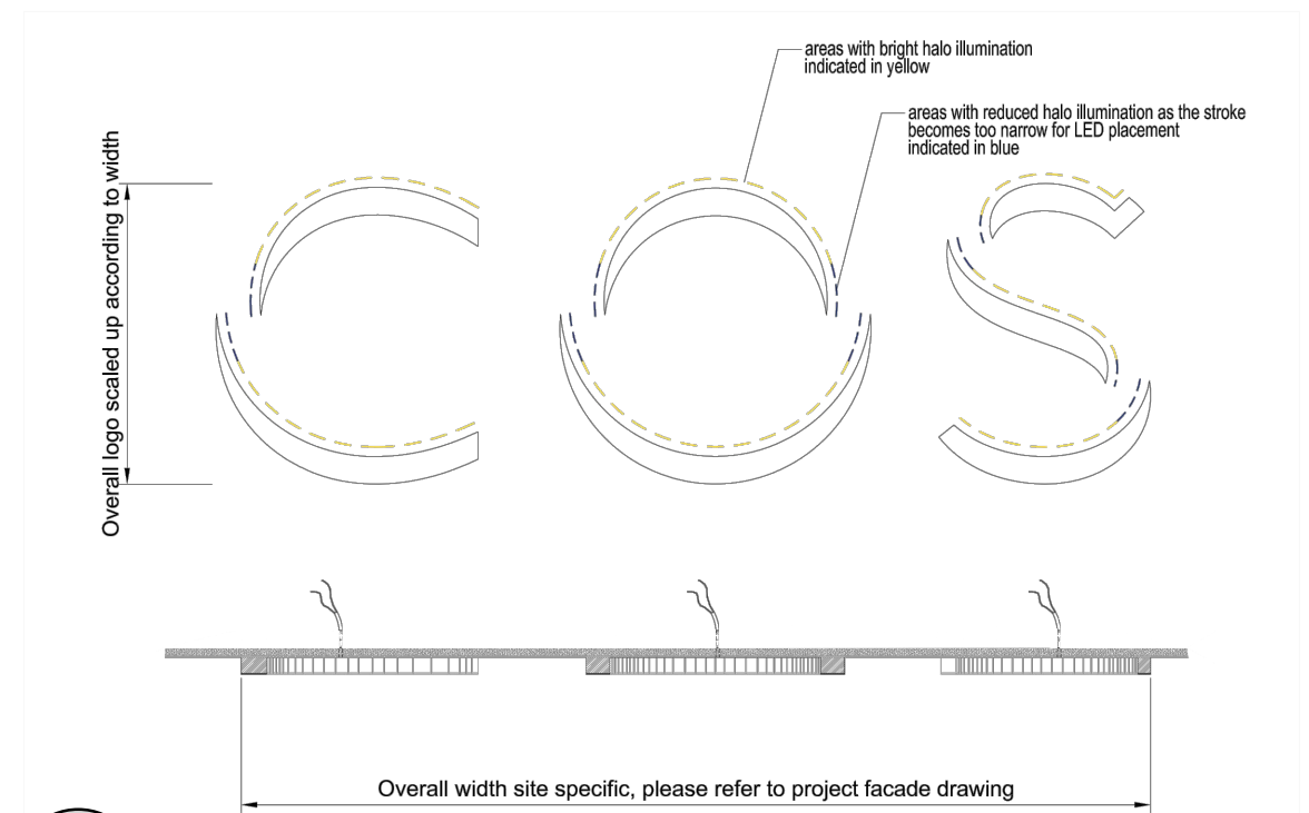
03 DETAIL. LIGHTING 404 N/A MAIN FASCIA SIGN
