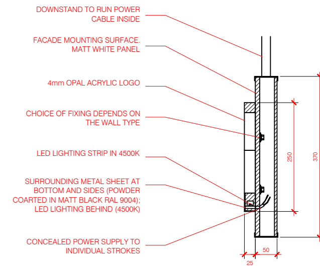
01 DETAIL. SECTION 404 1:10 MAIN FASCIA SIGN
