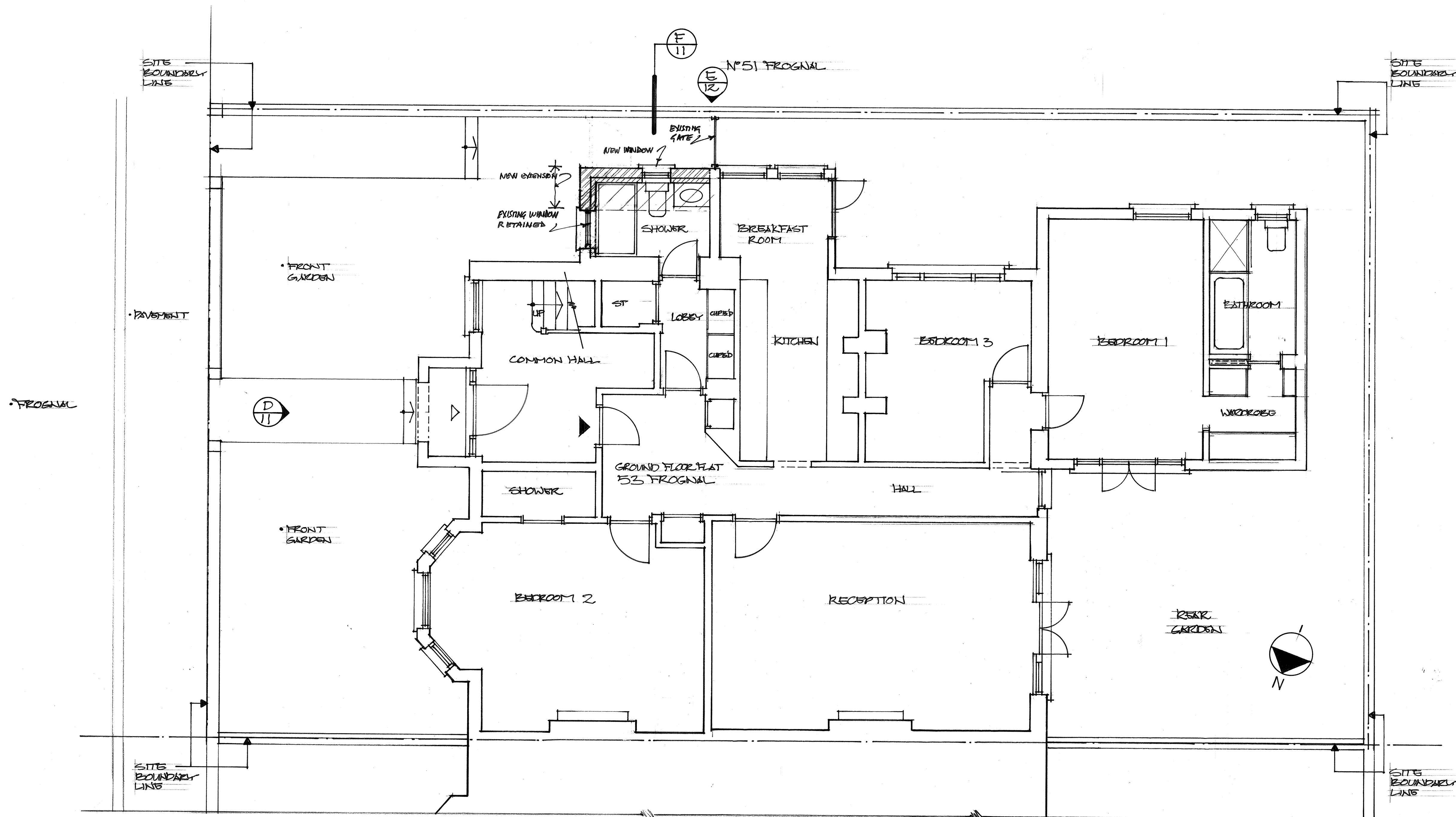
PROPOSED GROUND FLOOR AND SITE PLAN
