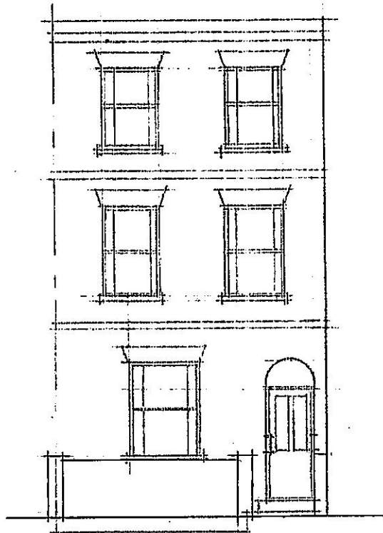
FRONT ELEVATION 1:100
