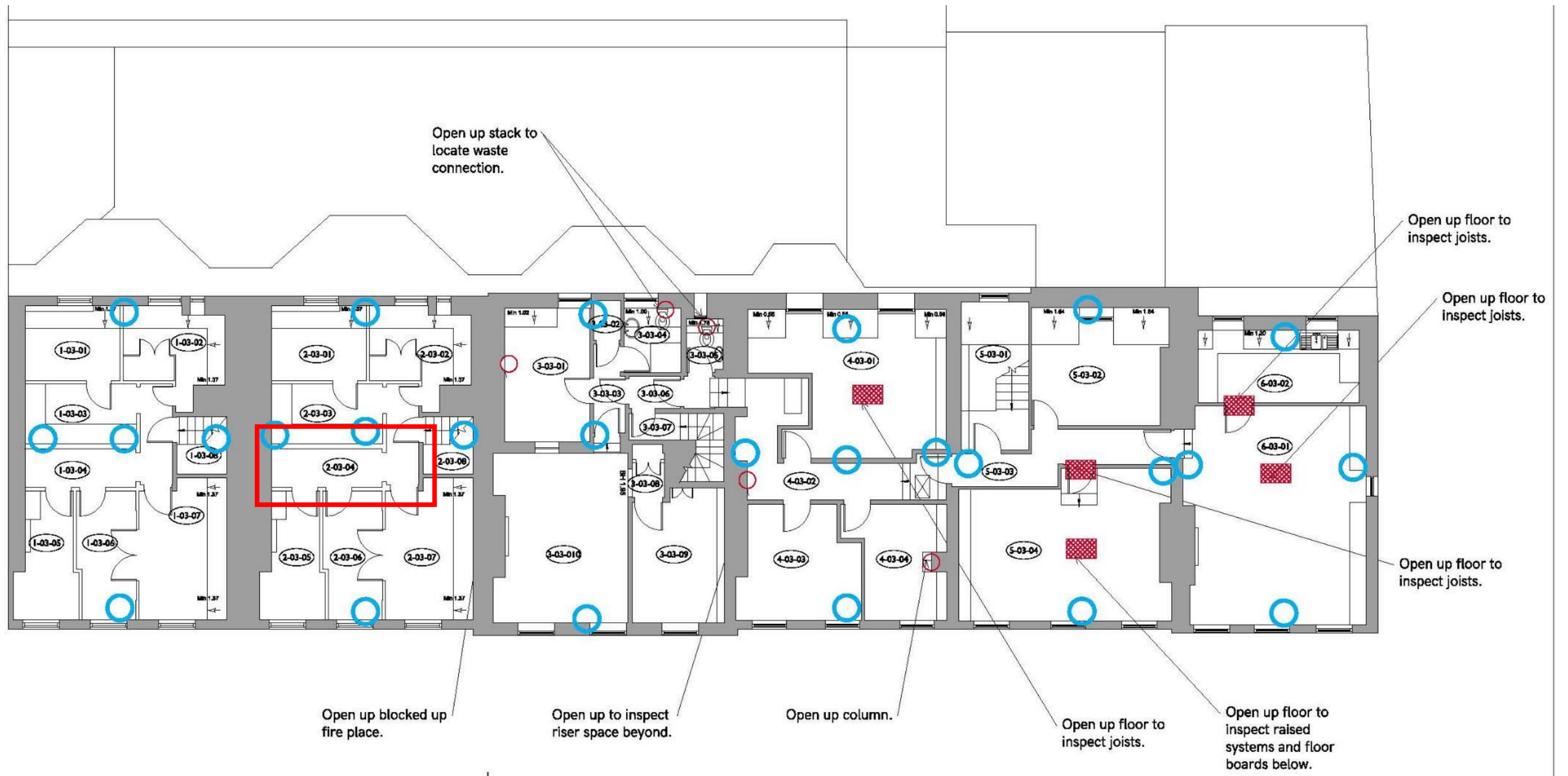
Figure 7: Number 20 - third floor plan key showing location of opening up photographs (2-03-04)
