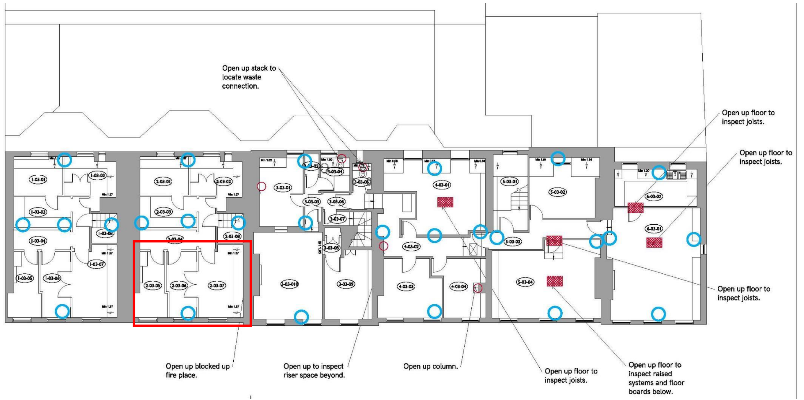
Figure 6: Number 20 - third floor plan key showing location of opening up photographs
