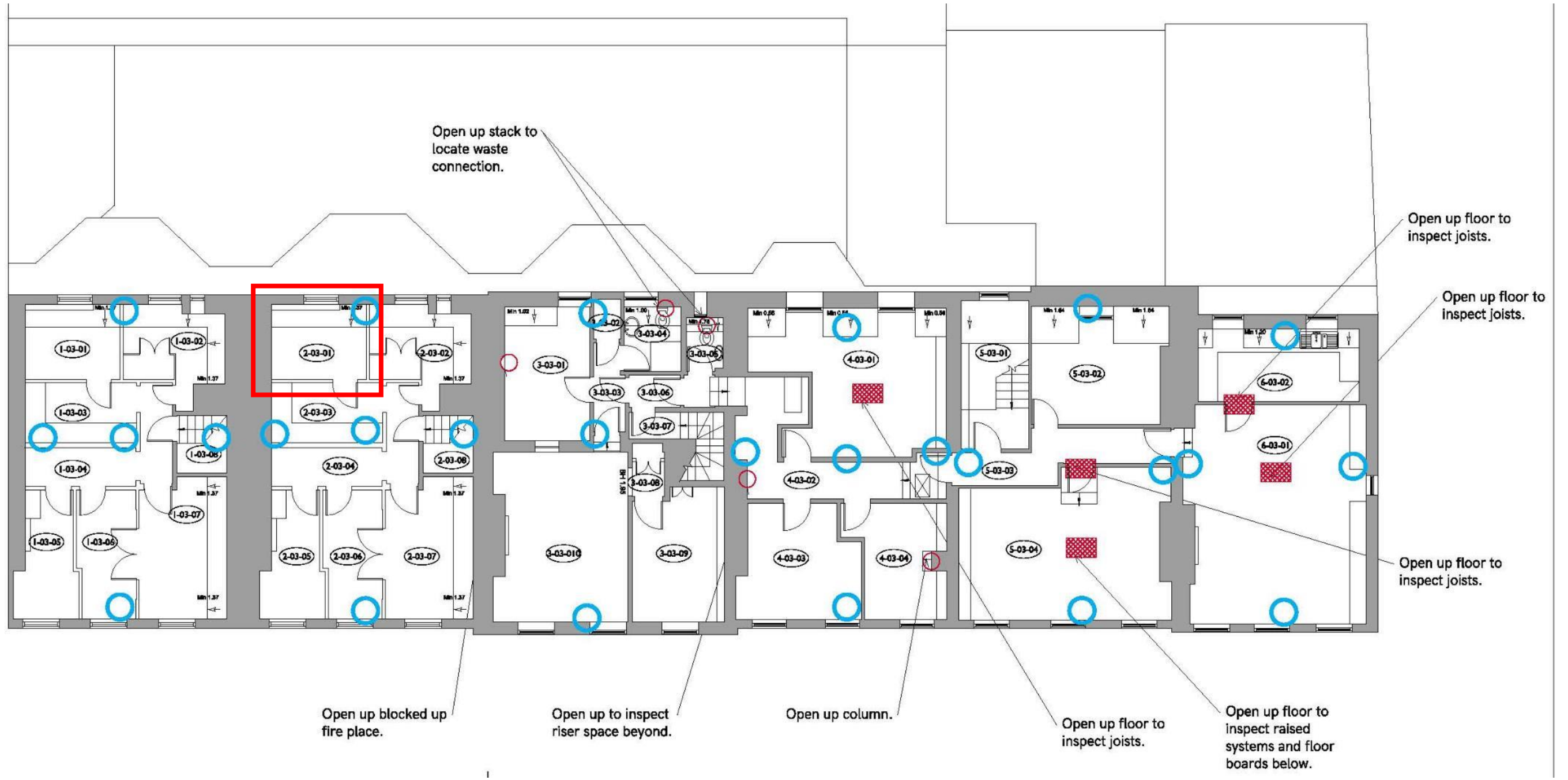
Figure 6: Number 20 - third floor plan key showing location of opening up photographs (2-03-01)
