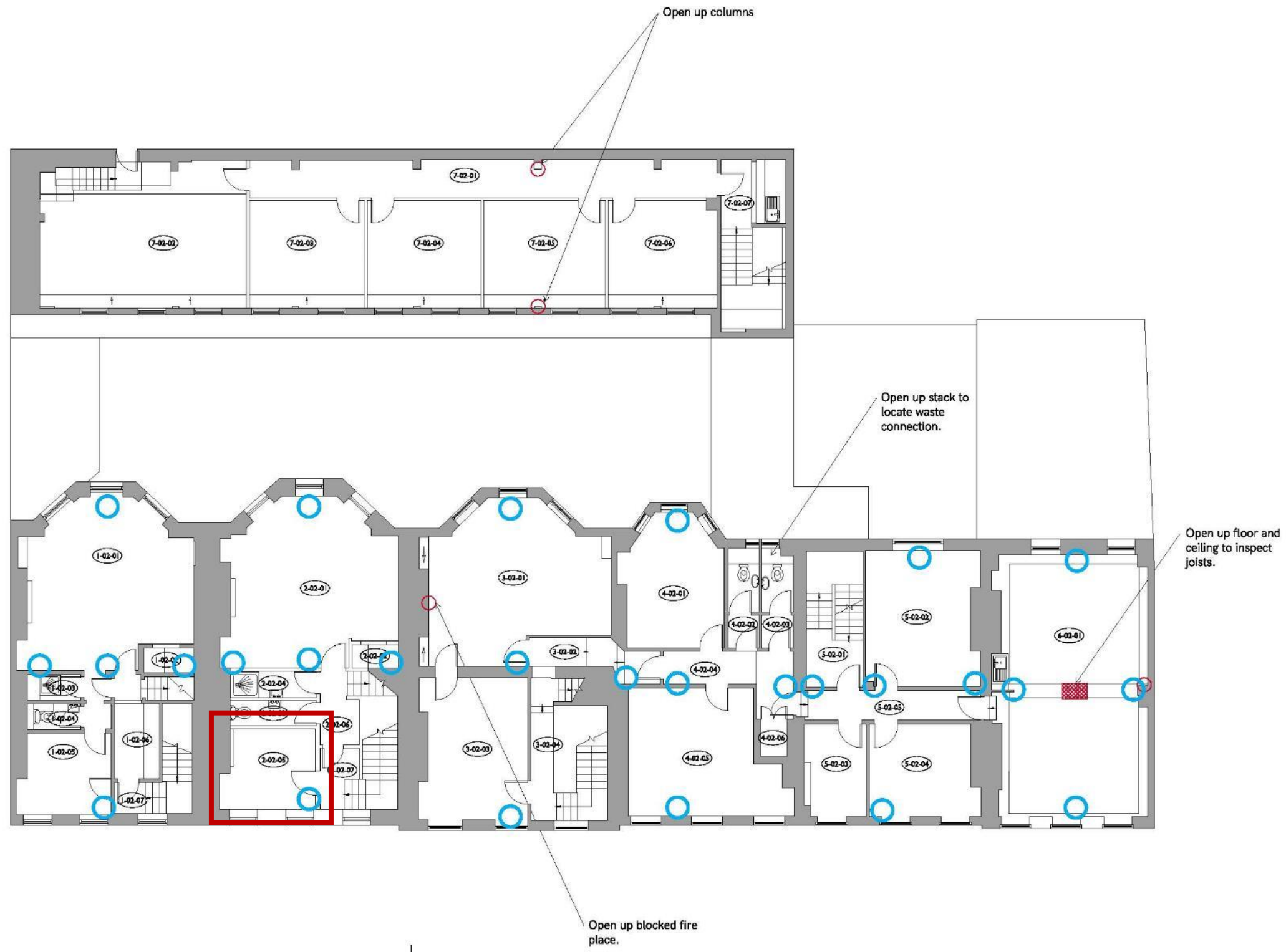
Figure 5: Number 20 - second floor plan key showing location of opening up photographs (2-02-05)
