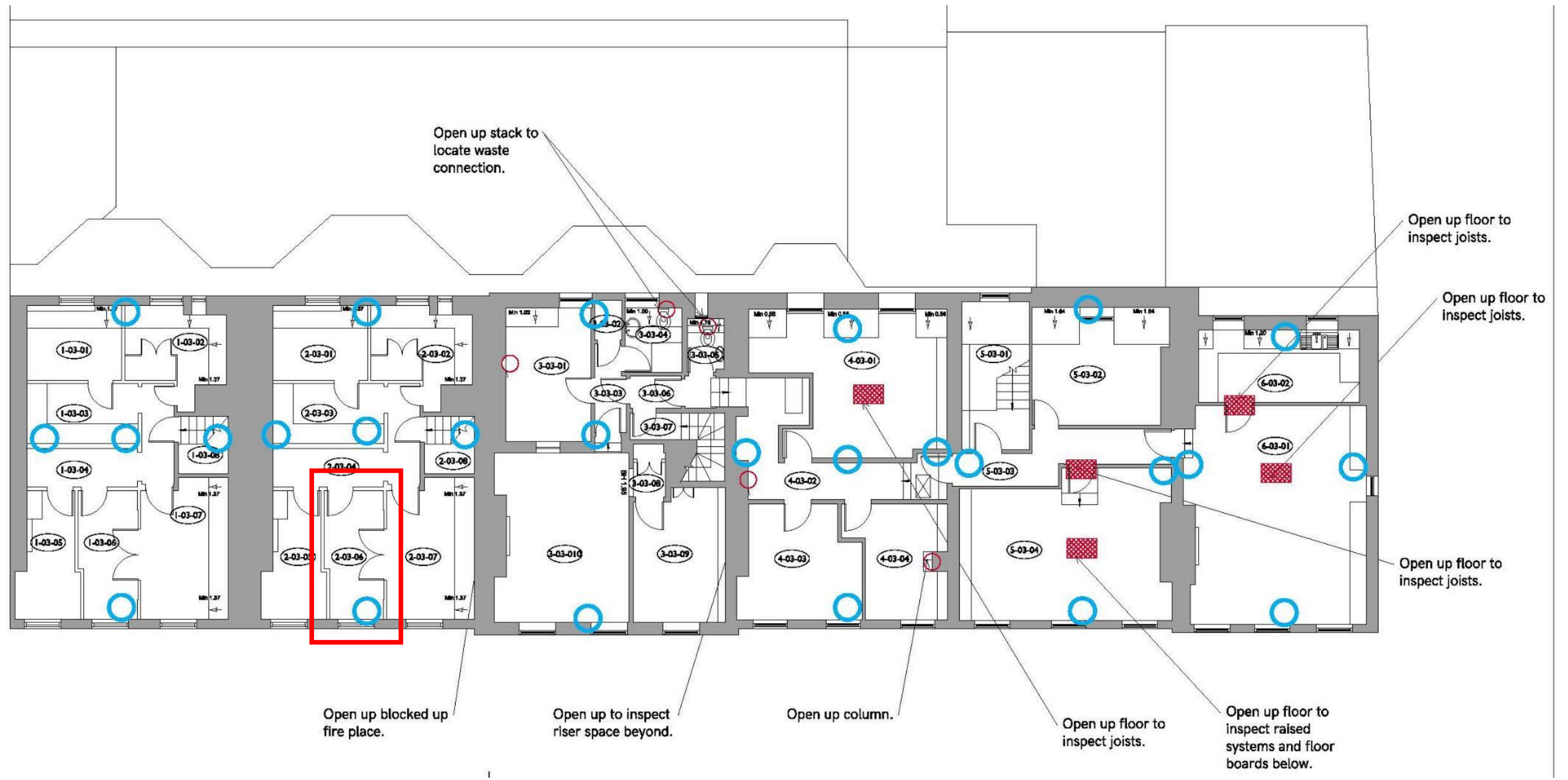
Figure 8: Number 20 - Third floor plan key showing location of opening up photographs (2-03-06)
