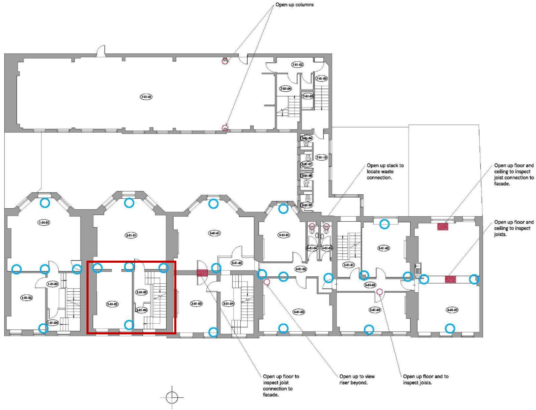
Figure 4: Number 20 - first floor plan key showing location of opening up
