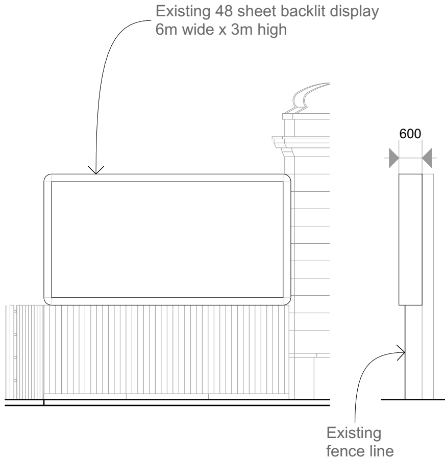
Existing West Elevation
