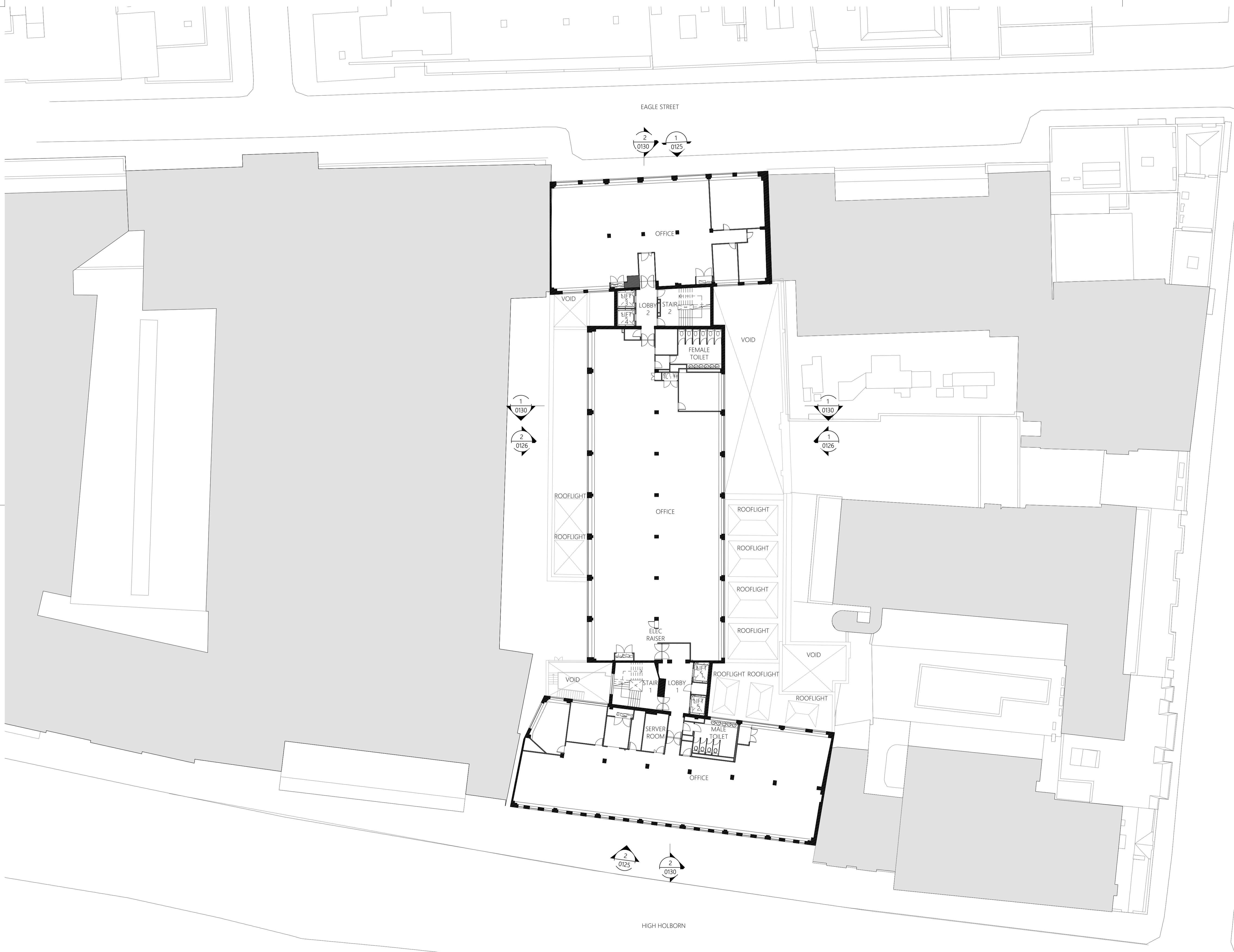
01 FOURTH FLOOR PLAN - EXISTING 1:200
