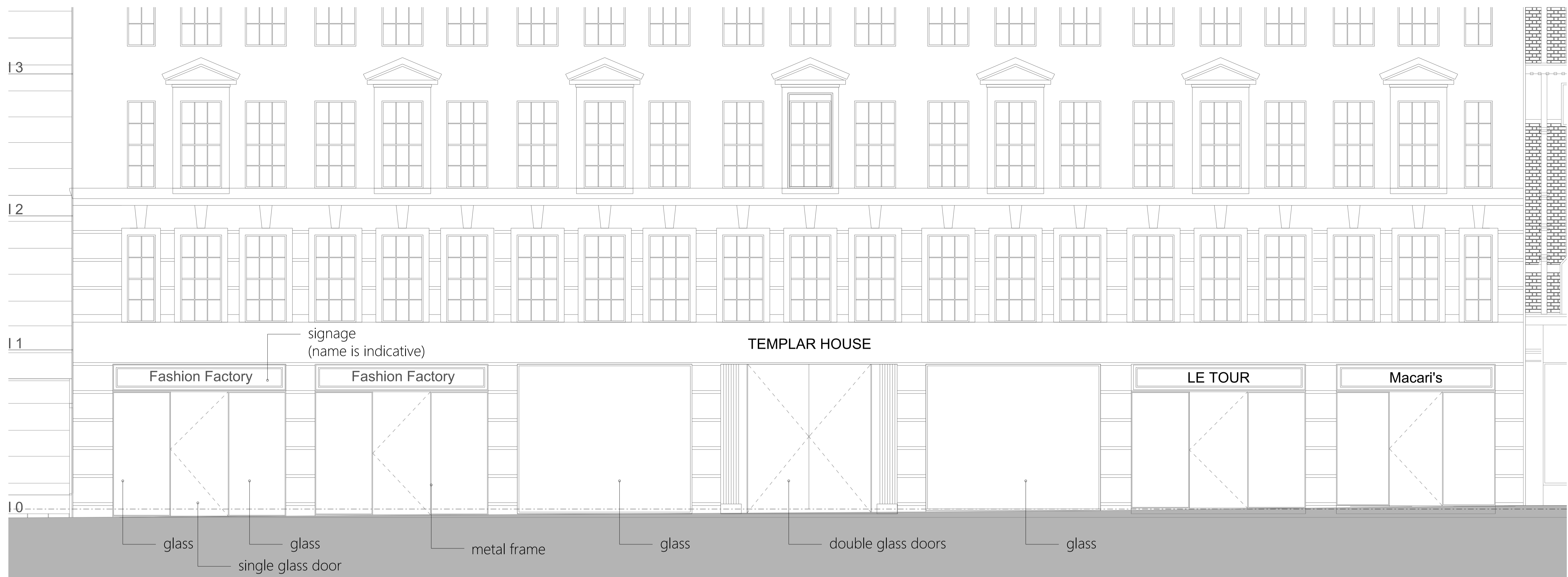
01 HIGH HOLBORN DETAIL ELEVATION 1:50
