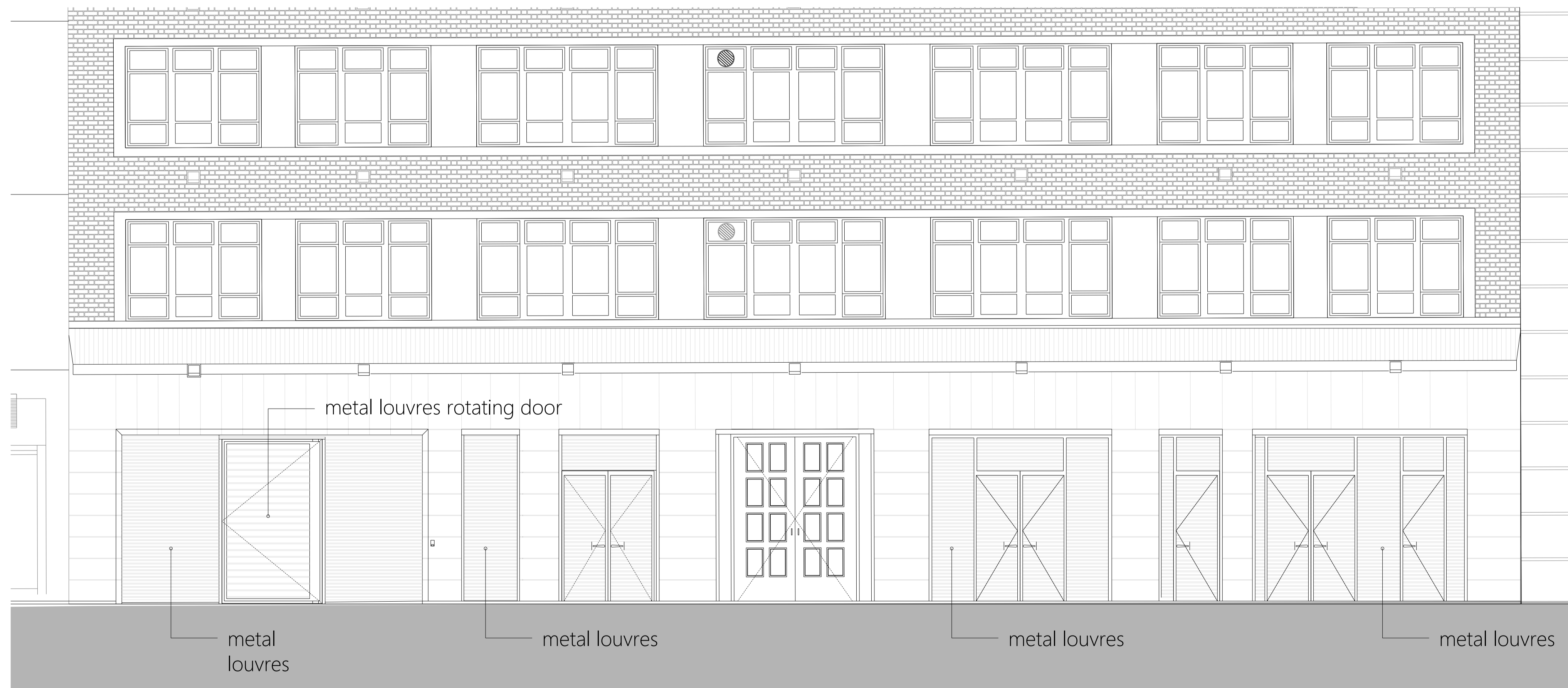
02 EAGLE STREET DETAIL ELEVATION 1:50
